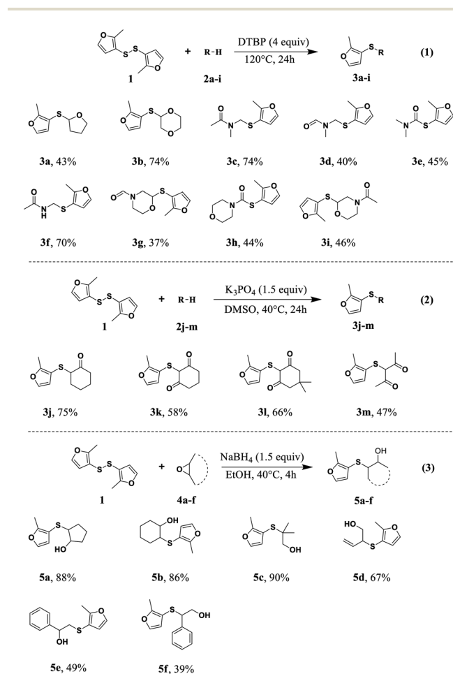
Scheme 1 Synthesis of 2-methyl-3-furyl sulfide derivatives.
