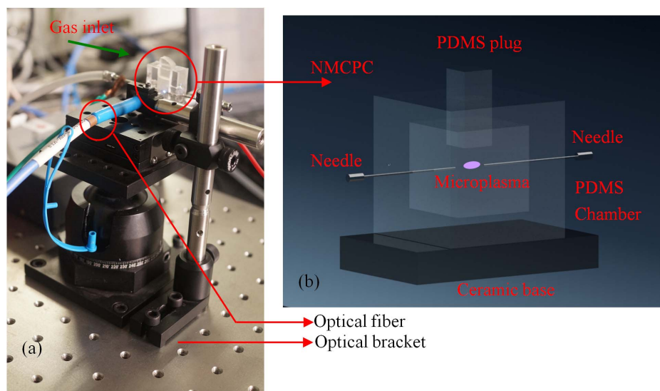
Figure 7 | Optical platform and NMPC configuration. (a) Photograph of the setup of the optical platform for the NMPC; (b) Diagrammatic representation for the component details of the NMPC.
