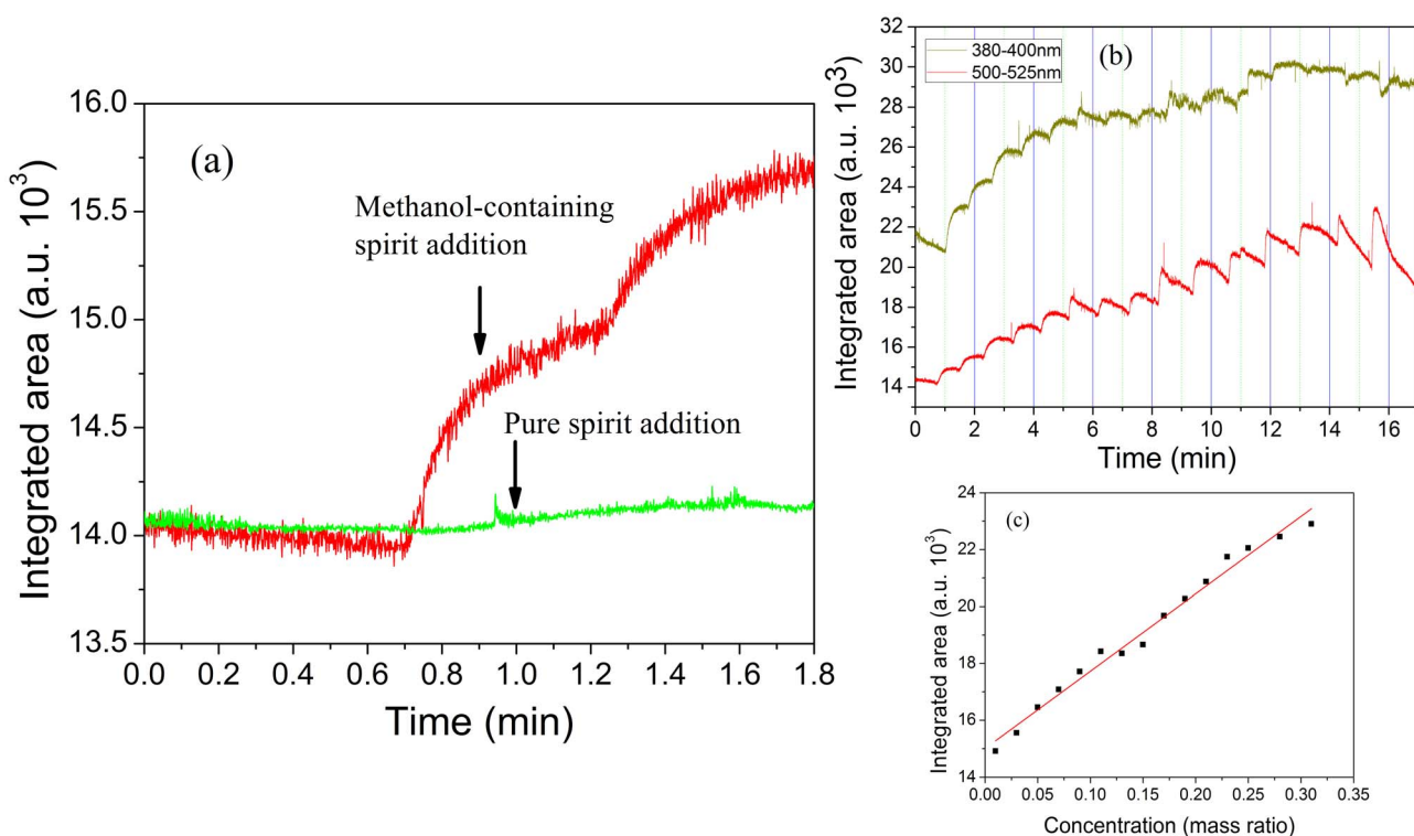
Figure 6 | Detection of the methanol-containing sample by time-response method. (a) Comparison of the response on introduction of the pure spirit (green line) and the methanol-containing spirit (red line) by monitoring the integrated area of R2 upon the elapsed time. A significant increase in intensity is evident upon methanol-containing sample addition. (b) Emission intensities as a function of time on gradient addition of various concentrations (0.01 to 0.31 mass ratios) of the methanol-containing alcohols by monitoring the integrated area of R1 and R2. (c) Calibration curve between the integrated area of R2 and the concentration of methanol in the alcohol samples. Lines are weighted linear fitting to the data obtained from 15 injected samples (5 \mu L for each).
