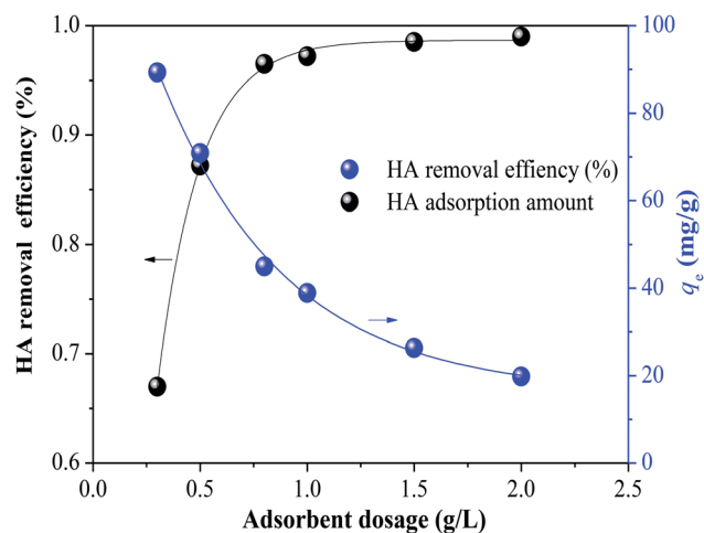
Fig. 2 Effect of dosage of SMZ6 adsorbent on HA adsorption. Experimental conditions: [HA]_0 = 40 \text{ mg L}^{-1} , contact time = 24 h, pH = 6.0, T = 20 \pm 1 \text{ }^\circ\text{C} .
