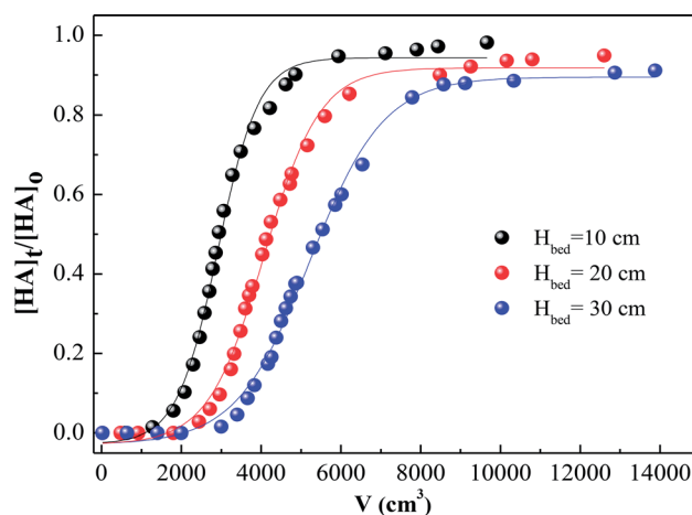
Fig. 11 Breakthrough curves for HA adsorption by SMZ6 fixed bed columns with different bed depths. Experimental conditions: flow rate = 4.0 mL min -1 , [HA]_0 = 40 mg L -1 , pH = 6.0, T = 20 \pm 1 °C.
