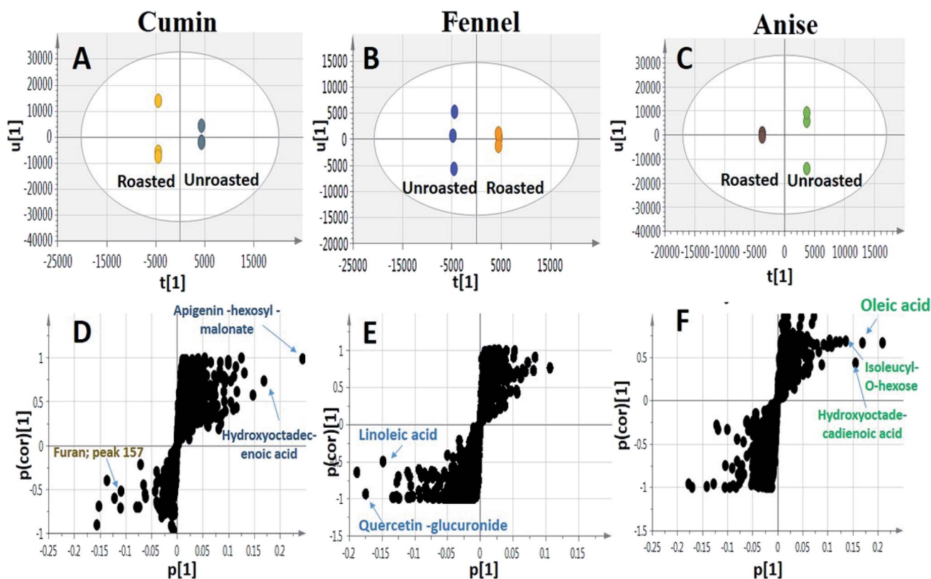
Fig. 4 UHPLC-MS based OPLS-DA score plots derived from modelling roasted against unroasted fruits (A–C). The S-plots (D–F) show the covariance p[1] against the correlation p(\text{cor})[1] of the variables of the discriminating component of the OPLS-DA models. Selected variables are highlighted in the S-plots and their biochemical pathway analysis are discussed in text.
