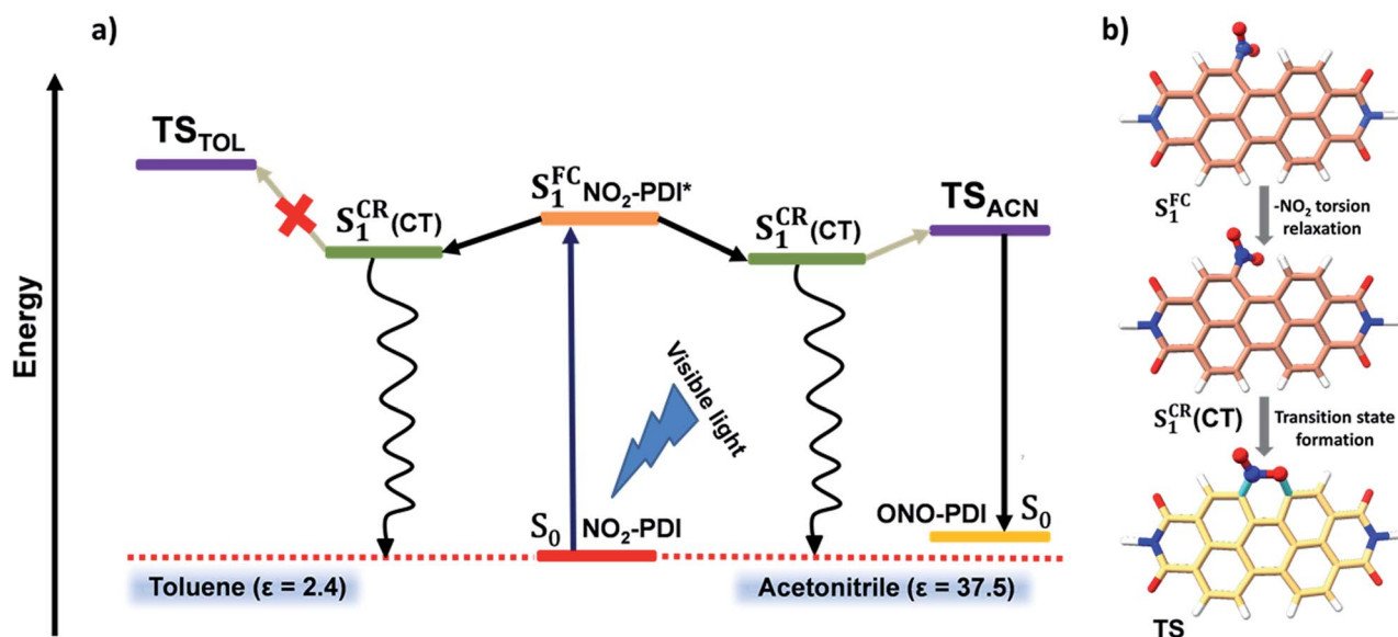
Fig. 6 (a) A pictorial illustration presenting a plausible kinetic mechanism explaining the excited-state dynamics and associated photochemistry of \text{NO}_2\text{-PDI} in the polar aprotic solvent acetonitrile and non-polar solvent toluene. Here, the S_0 state represents the ground state of \text{NO}_2\text{-PDI} and \text{ONO-PDI} , the S_1^{\text{FC}} state represents the Franck–Condon state of \text{NO}_2\text{-PDI} , and the S_1^{\text{CR}} (CT) state is a long-lived transient species observed in nsTA measurements, representing the conformationally relaxed singlet excited-state of \text{NO}_2\text{-PDI} having charge-transfer character. (b) Optimized geometries showing the transition from the S_1^{\text{FC}} state first to the S_1^{\text{CR}} (CT) state and finally to the six-membered TS through the nitro-aromatic torsion relaxation pathway computed at the CAM-B3LYP/6-311++G(d,p) level (the –R group was replaced by a –H atom to reduce the computational cost and increase clarity).
