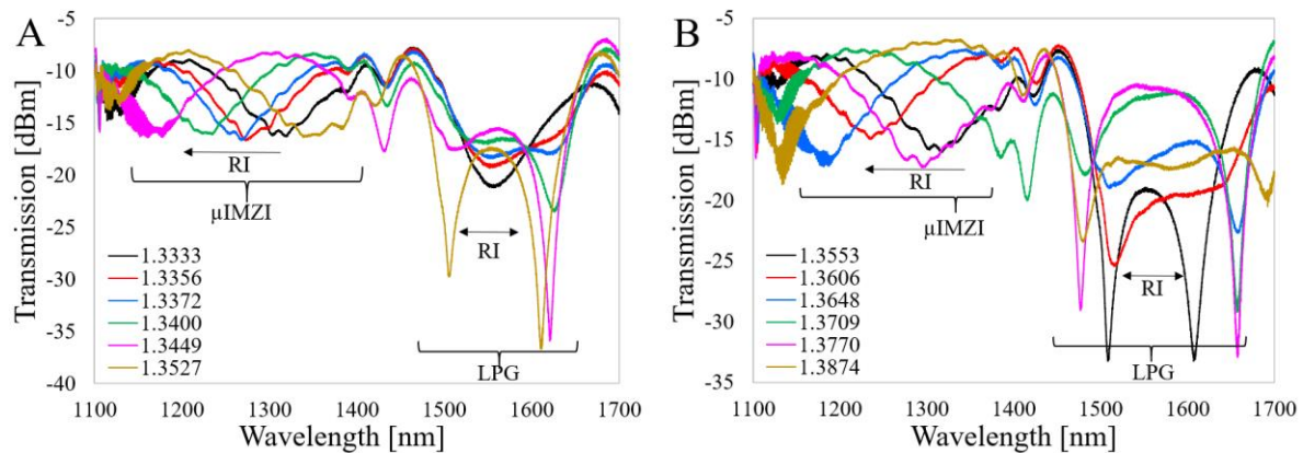
Figure 5. Spectral response of the LPG- \mu MZI structure to RI in ranges: (A) from 1.3333 to 1.3527 RIU and (B) from 1.3553 to 1.3874 RIU. The effects corresponding to the LPG and \mu MZI are marked in the figures.
