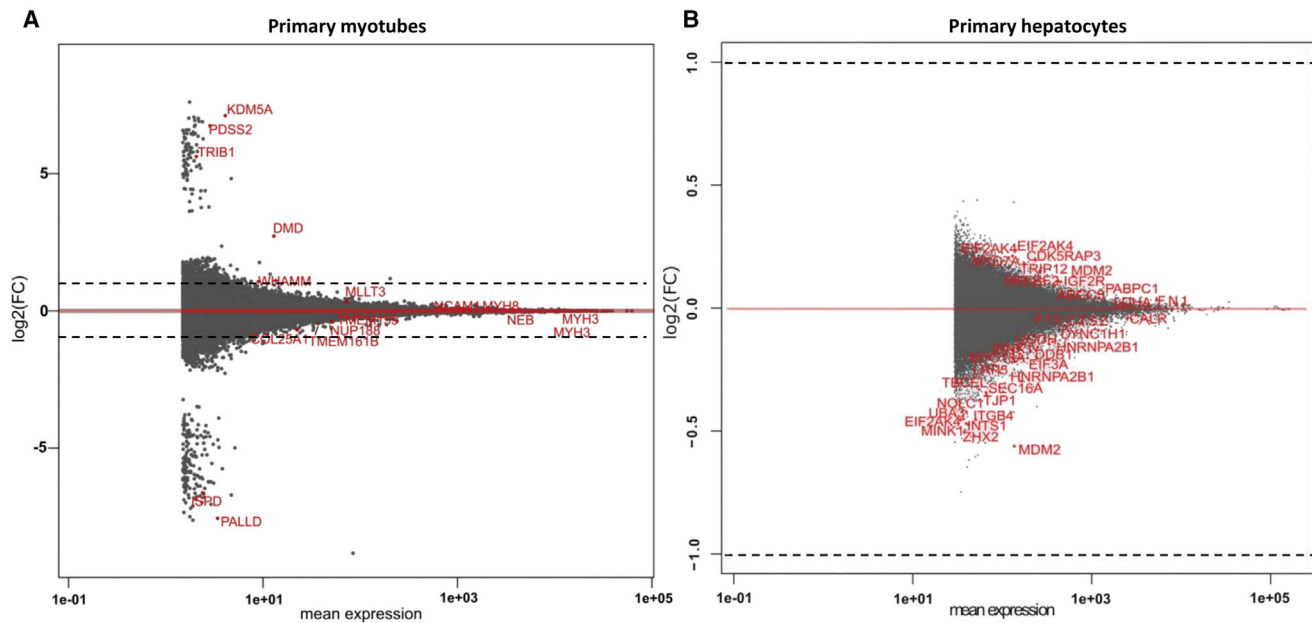
Figure 6. Exon Junction Usage Analyzed Using DEXseq
