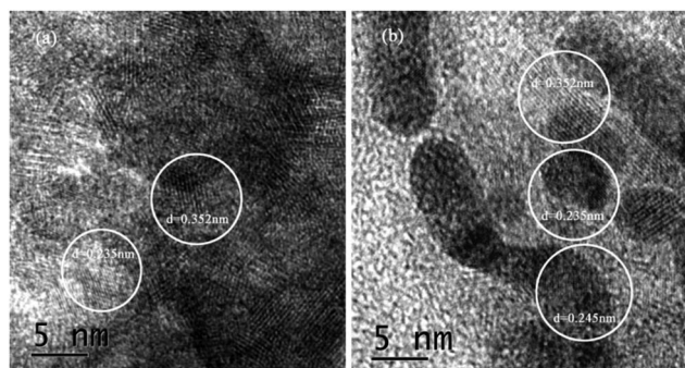
Fig. 4 TEM images of samples (a) {001}TiO 2 , (b) 1 : 10.
