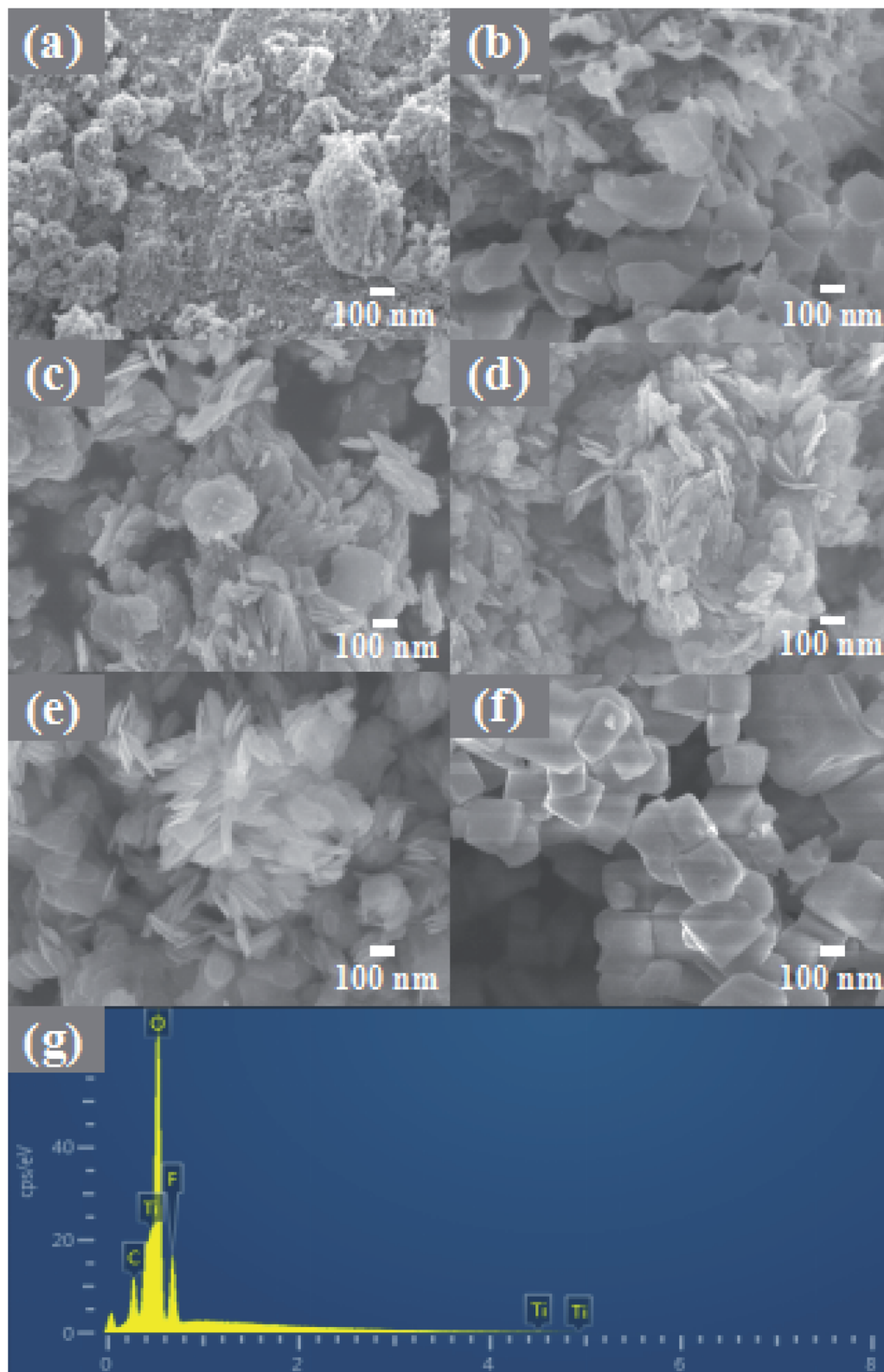
Fig. 2 The high-magnification FE-SEM images of (a) TiO 2 , (b) 4-TF, (c) 6-TF, (d) 8-TF, (e) 10-TF and (f) TiOF 2 ; EDS images of 8-TF (g).
