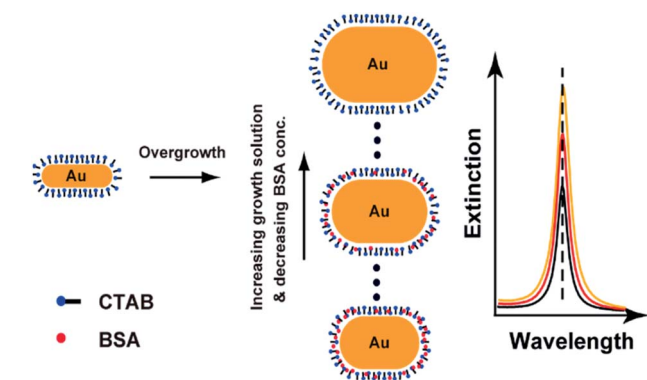
Scheme 1 Overgrowth of AuNRs using a binary surfactant mixture consisting of BSA and CTAB. Tailoring the optical cross sections of AuNRs at a fixed target LSPR wavelength can be accomplished by controlling the combinations of BSA concentrations and the volumes of the growth solution.
