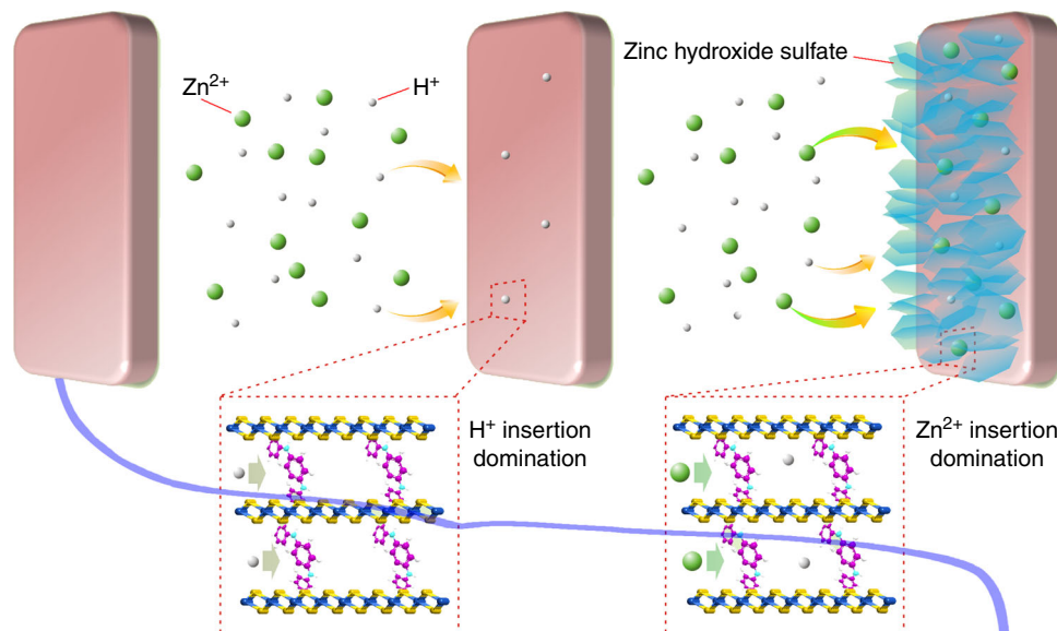
Fig. 5 Diagram showing the sequential insertion of H + and Zn 2+ . During the first discharge platform, H + insertion into polyaniline (PANI)-intercalated MnO 2 nanolayers dominates the electrode reaction, which gradually decreases H + concentration around the electrode. With a sustained decrease of H + , Zn 2+ insertion dominates the electrochemical reaction, raising the second discharge platform; meanwhile, the sustained decrease of H + concentration leads to the formation of zinc hydroxide sulfate on the electrode surface
