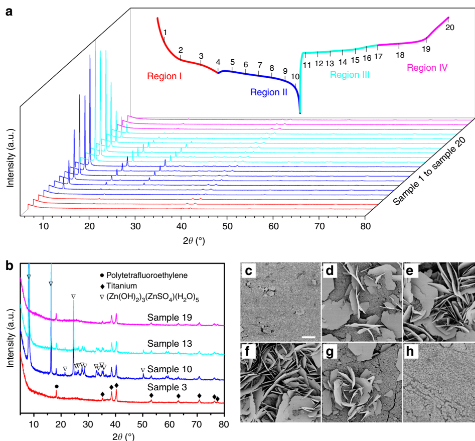
Fig. 3 Structure evolution of polyaniline-intercalated \text{MnO}_2 electrode during cycling. a Evolution of ex situ X-ray powder diffraction (XRD) patterns during the charge/discharge process (the vertical bars denoted with consecutive numbers indicate the locations where the XRD patterns were recorded). b Selected ex situ XRD patterns from a (corresponding to the XRD patterns denoted with 3, 10, 13, and 19 in a ), which represent the typical XRD pattern in each corresponding charge/discharge region. c–h Scanning electron microscopy (SEM) images for morphologic evolution of electrode during cycling (the SEM images were taken at the locations indicated by vertical bars 3, 5, 10, 12, 16, and 20 in a , respectively). Scale bars, c–h 10 \mu\text{m} , respectively (the magnification is the same for images c–h )
