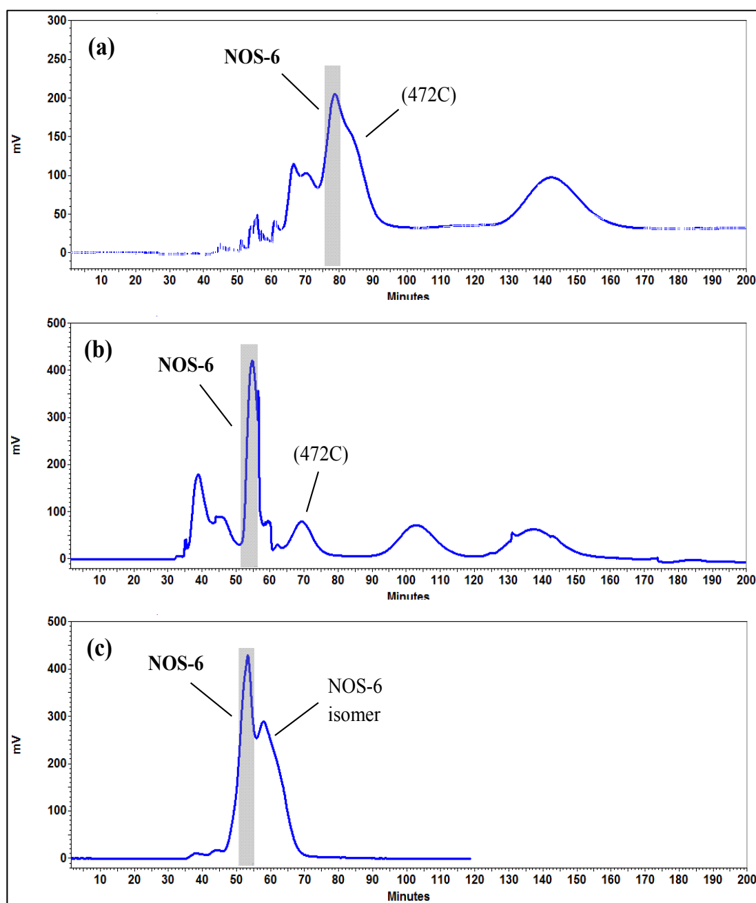
Figure 3. (a) HPCCC chromatogram of acetone-treated crude extract of Nostoc sp. Two phase solvent system: HEMWat, 4:5:4:5, v/v/v/v; mobile phase: lower phase; elution mode: reverse phase; flow rate: 1 mL/min; detection: 280 nm. (b) First-step HPCCC chromatogram of acetone-treated crude extract of Nostoc sp. Two phase solvent system: HEMWat, 4:5:4:5, v/v/v/v; stationary phase: neutral upper phase; mobile phase: base lower phase (1% NH 3 in lower phase, pH 8.7); elution mode: reverse phase; flow rate: 1 mL/min; detection: 280 nm; 472C: contaminant (ion at m/z 472 from HPLC/ESI-HRMS analysis). (c) Second-step HPCCC chromatogram of target fraction. Two phase solvent system: HEMWat, 4:5:4:5, v/v/v/v; stationary phase: neutral upper phase; mobile phase: neutral lower and base lower phase (1% NH 3 in lower phase, pH 8.7) as mobile phase with a linear gradient elution exchanged from 100:0 for 70 min and then to 0:100 for 130 min; elution mode: reverse phase; flow rate: 0.8 mL/min; detection, 280 nm.
