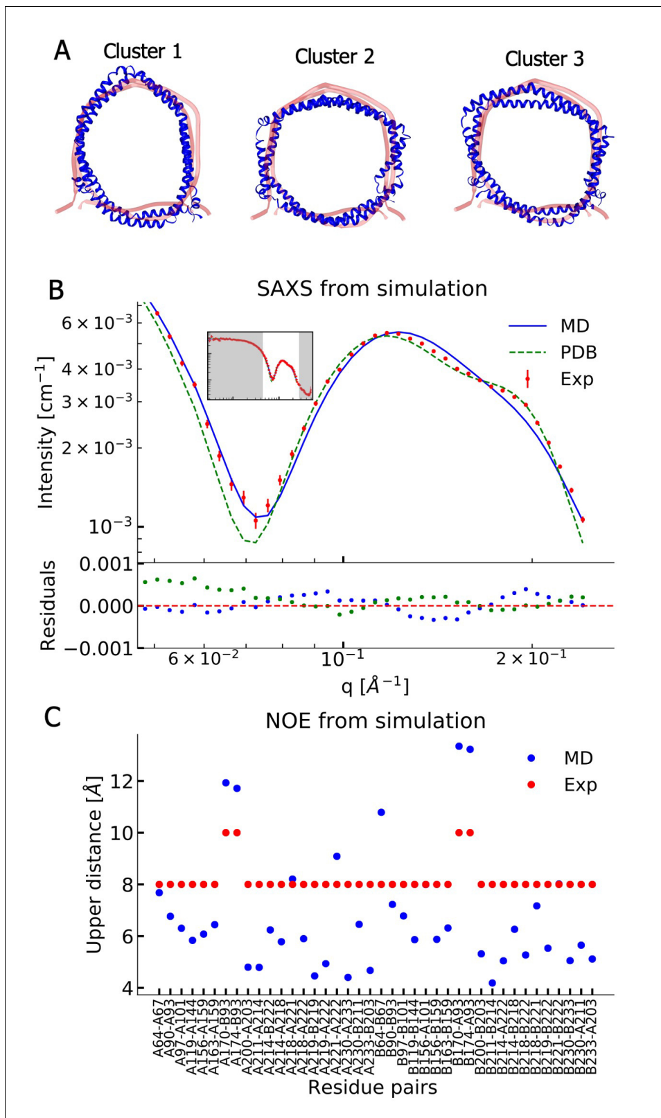
Figure 2. Comparing MD simulations with experiments. (A) Visualization of the conformational ensemble from the MD simulation by clustering (blue). Only the protein parts of the nanodisc are visualized while the lipids are left out to emphasize the shape. The top three clusters contain 95% of all frames. The previous NMR/EPR-structure is shown for comparison (red). (B) Comparison of experimental standard solution SAXS data (red) and SAXS calculated from the simulation (blue). Green dotted line is the back-calculated SAXS from the integrative NMR/EPR-structure (labelled PDB). Residuals Figure 2 continued on next page
