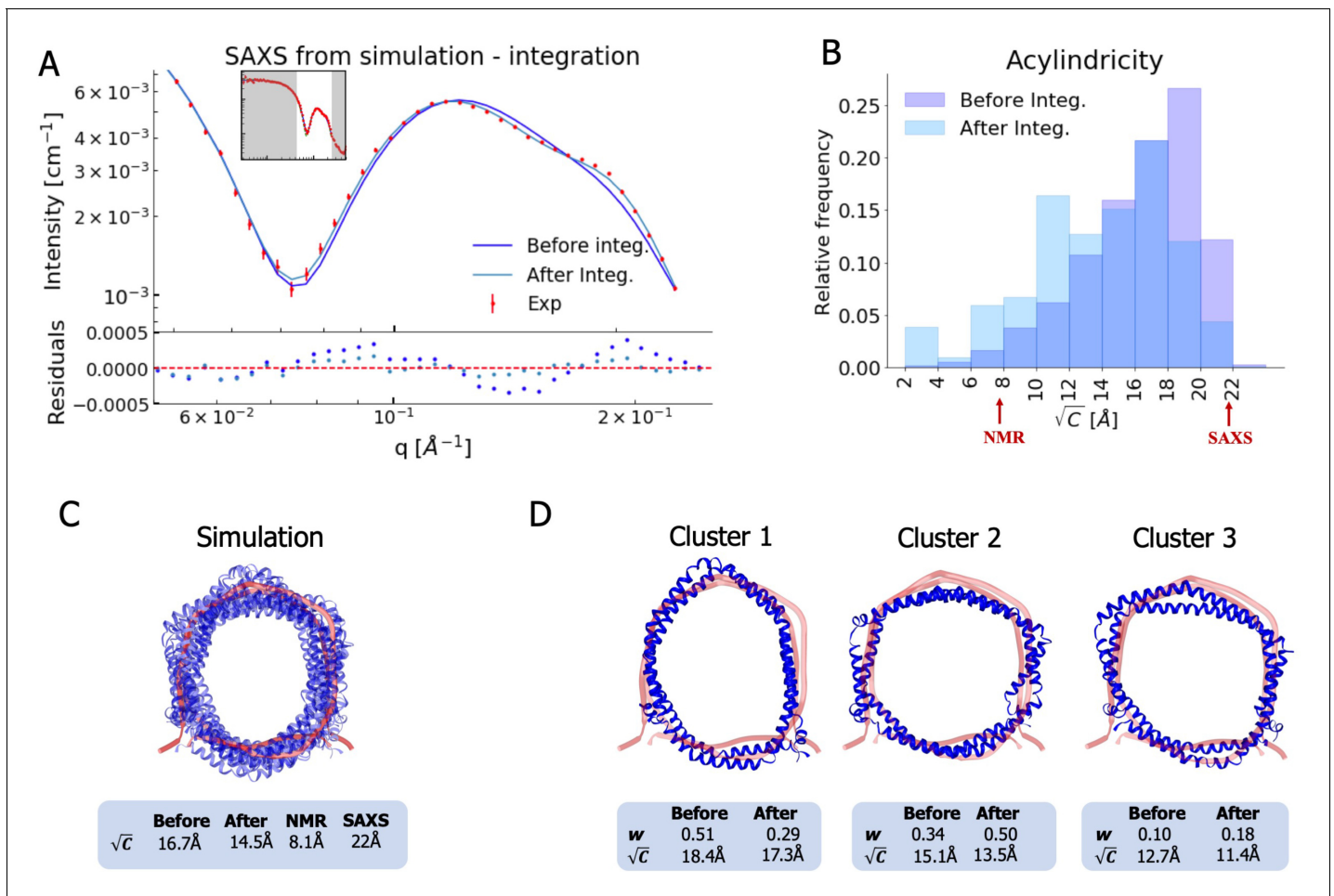
Figure 3. Integrating simulations and experiments. (A) SAXS data calculated from the simulation before and after reweighting the ensemble using experimental data. Only the high q -range is shown as the discrepancy between simulation and experiments are mainly located here (for the entire q -range see Figure 3—figure supplement 1 ). Agreement with the NOEs before and after integration are likewise shown in Figure 3—figure supplement 2 . (B) Histogram of the acylindricity of the simulations ( \sqrt{C} ) both before integration (dark blue) and after integration (light blue). (C) Visualization of the conformational ensemble showing structures sampled every 100 ns in cartoon representation (blue), the original NMR/EPR structure is shown in rope representation for comparison (red). The table below shows the acylindricity of the entire conformational ensemble before and after integration and compared to the original NMR/EPR (NMR) structure and the SAXS/SANS model fit. (D) Weights and acylindricity of the three main clusters of the MD simulation (blue) before and after integration.
