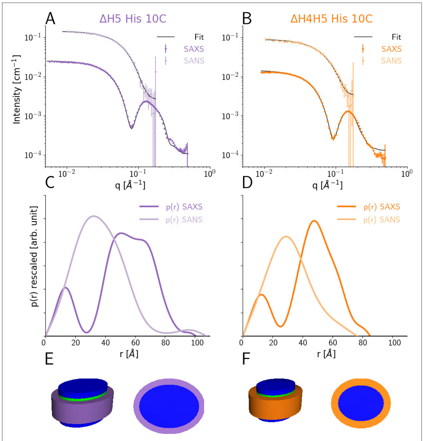
Figure 1. SEC-SAXS and SEC-SANS analysis of nanodiscs. (A) SEC-SAXS (dark purple) and SEC-SANS (light purple) for \Delta\text{H5} -DMPC nanodiscs at 10^\circ\text{C} . The continuous curve show the model fit corresponding to the geometric nanodisc model shown in E. (B) SEC-SAXS (dark orange) and SEC-SANS (light orange) data for the \Delta\text{H4H5} -DMPC nanodiscs at 10^\circ\text{C} . (C,D) Corresponding pair-distance distribution functions. (E, F) Fitted geometrical models for the respective nanodiscs (drawn to scale relative to one another).
