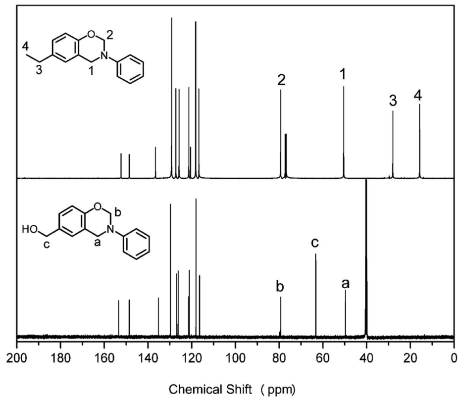
Fig. 2 ^{13}\text{C} NMR spectra of p\text{HBA-a} (in \text{DMSO-}d_6 ) and p\text{EPH-a} (in \text{CDCl}_3 ).
