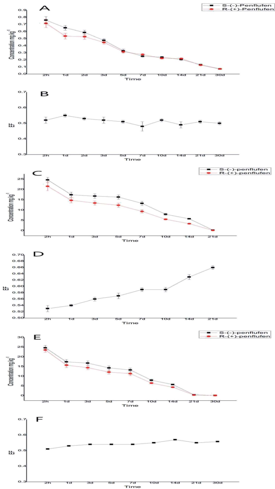
Fig. 4 Stereoselective degradation of penflufen on wheat plant, spinach, and Chinese cabbage (wheat plants: A and B; spinach: C and D; Chinese cabbage: E and F).
