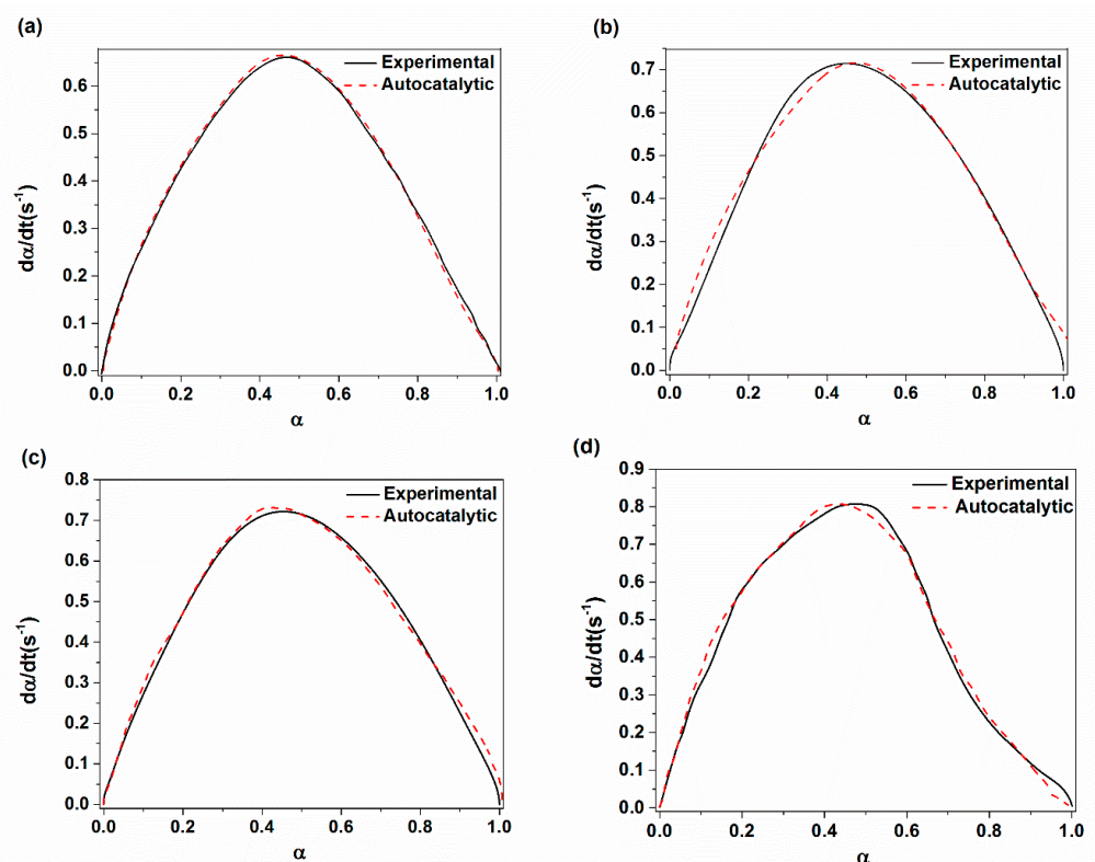
Figure 10. Comparison of experimental conversion rate with predicted ones through using autocatalytic approach and isothermal DSC curves with respect to cure conversion parameter for: (a) XE15; (b) XE15H3; (c) XE15H5; (d) XE15H7
