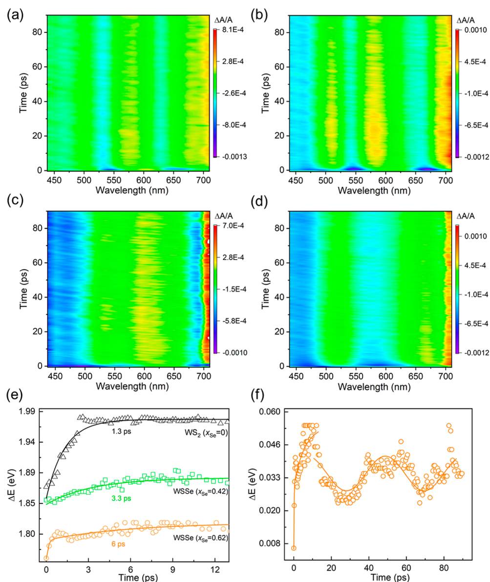
Figure 7. TA ( \Delta A/A ) profile of (a) WS 2 , (b) WSSe ( x_{Se} = 0.42 ), (c) WSSe ( x_{Se} = 0.62 ), and (d) WSe 2 nanotubes (up to 10 and 90 ps delay). Note the oscillating signal \sim 690 nm for WSSe ( x_{Se} = 0.42 ) nanotubes, which is not present in other materials. (e) Temporal dynamics of exciton-polariton transitions in the ultrafast time scale for WS 2 , WSSe ( x_{Se} = 0.42 ), and WSSe ( x_{Se} = 0.62 ) nanotubes. (f) Oscillating dynamics of incoherent to coherent transition in WSSe ( x_{Se} = 0.62 ) nanotubes.
