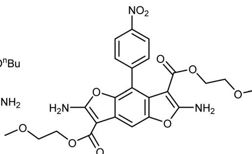
42: ( IC_{50} > 200 \mu\text{M} )
