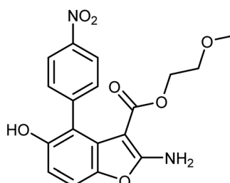
40: ( IC_{50} = 142 \mu\text{M} )
