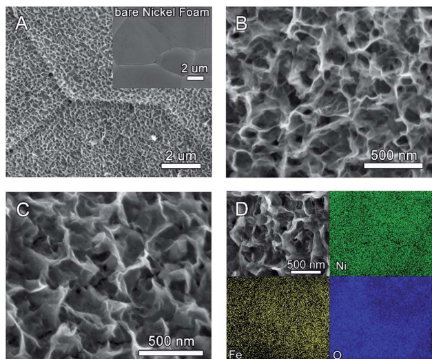
Fig. 1 (A and B) SEM images of different magnifications for Ni(OH) 2 /NF nanosheets grown from nickel foam (inset is SEM image of a bare nickel foam). (C) SEM and (D) SEM-EDX mapping images of the Ni(OH) 2 -Fe/NF electrode.
