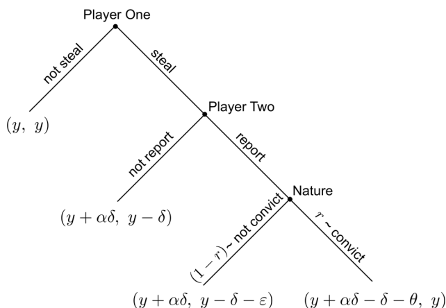
Figure 1. The adversarial interaction represented in a game tree. The final payoffs in the format (player one, player two) are given at the terminal nodes.
