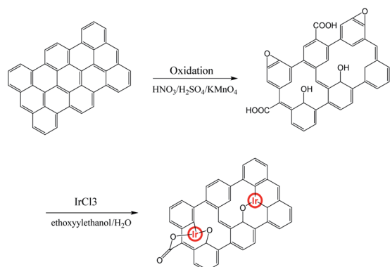
Scheme 1 Illustration of the methods used for preparing graphene oxide–iridium complex.
