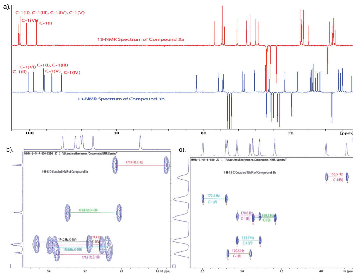
Fig. 3 (a) Comparison of ^{13}\text{C} -NMR spectra of compounds 3a (150 MHz, C 6 D 6 ) and 3b (150 MHz, CDCl 3 ); (b) ^{13}\text{C} - ^1\text{H} coupled 2D-NMR spectrum of compound 3a (C 6 D 6 ); (c) ^{13}\text{C} - ^1\text{H} coupled 2D-NMR spectrum of compound 3b (CDCl 3 ).
