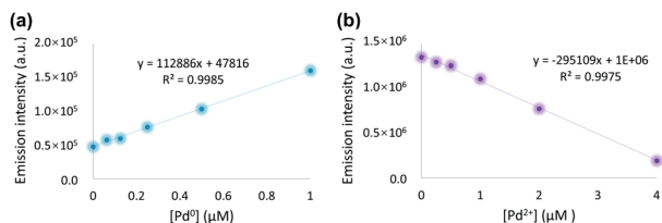
Fig. 4 Fluorescence analysis of PPIX-L2 against various concentrations of Pd 0 and Pd 2+ in MeOH for the determination of detection limit. (a) Linear correlation between coumarin fluorescence intensity of 5 μM PPIX-L2 at 440 nm and [Pd 0 ]. Fluorescence intensity was recorded at 2 hours after the addition of Pd 0 ( \lambda_{\text{ex}} = 361 nm). (b) Linear correlation between porphyrin fluorescence intensity of 2 μM PPIX-L2 at 631 nm and [Pd 2+ ]. Fluorescence intensity was recorded at 1 hour after the addition of Pd 2+ ( \lambda_{\text{ex}} = 400 nm).
