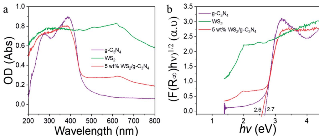
Fig. 5 (a) UV-vis diffuse reflection spectra of pure \text{g-C}_3\text{N}_4 , \text{WS}_2 and 5 wt% \text{WS}_2/\text{g-C}_3\text{N}_4 composite; (b) corresponding bandgap of pure \text{g-C}_3\text{N}_4 , \text{WS}_2 and 5 wt% \text{WS}_2/\text{g-C}_3\text{N}_4 composite estimated from Kubelka–Munk equation.
