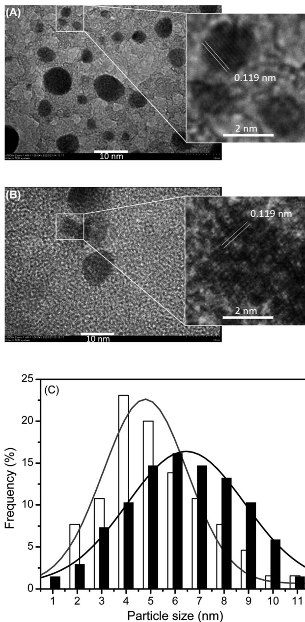
Fig. 4 The HRTEM images of (A) AcpySB-Ag 2 S QDs and (B) TGA-Ag 2 S QDs, showing their lattice fringes with spacing of 0.119\text{ nm} , corresponding to the (-112) plane of acanthite Ag 2 S, and (C) the particle size distribution of AcpySB-Ag 2 S QDs (white bars) and TGA-Ag 2 S QDs (black bars) along with their respective best-fit Gaussian curve.
