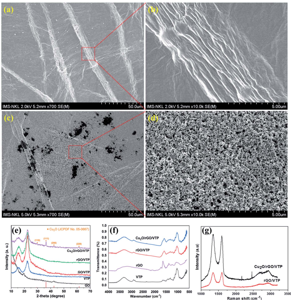
Fig. 2 Characterizations of the \text{Cu}_2\text{O}/\text{rGO}/\text{VTP} photocatalyst: (a and b) SEM images of \text{GO}/\text{VTP} at a magnification of 700\times (a) and 10k\times (b); (c and d) SEM images of \text{Cu}_2\text{O}/\text{rGO}/\text{VTP} at 700\times (c) and 10k\times (d); (e) XRD spectra of the samples; (f) FTIR spectra of the samples; (g) Raman spectra of the samples.
