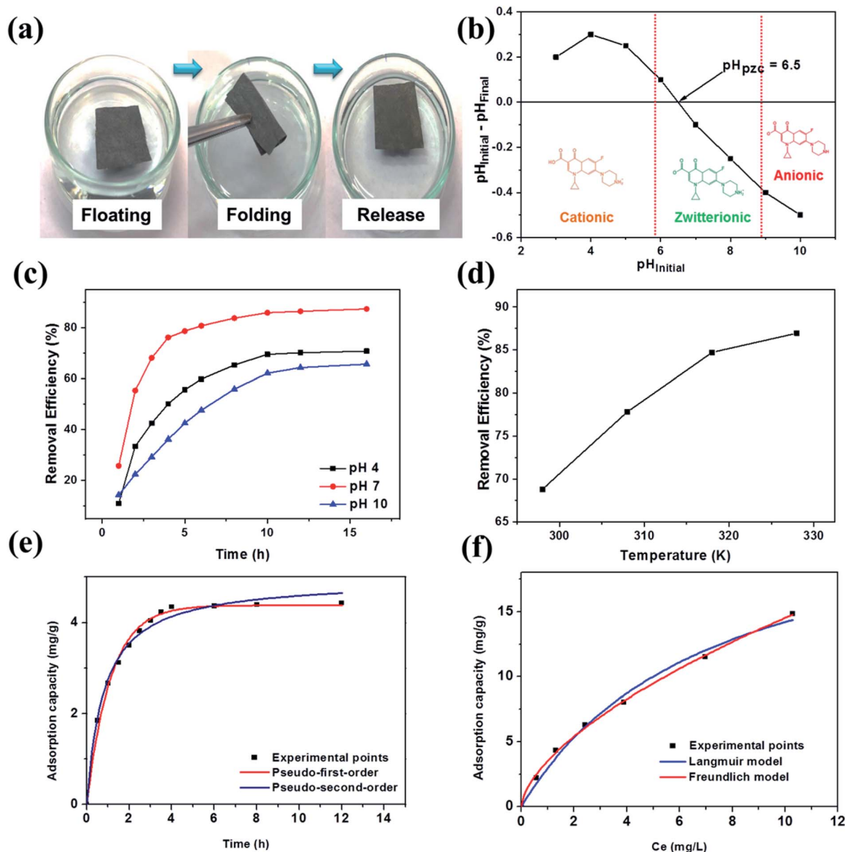
Fig. 3 Adsorption of CIP onto \text{Cu}_2\text{O}/\text{rGO}/\text{VTP} : (a) illustration of the highly flexible and floatable catalyst membrane; (b) the point of zero charge (PZC) of the catalyst; (c) the effects of pH on the removal efficiency of CIP by the catalyst; (d) the effects of temperature on the removal efficiency of CIP by the catalyst; (e) plot of fitting between the experimental data to the pseudo-first-order and the second-order adsorption models; (f) plot of fitting between the experimental data to the Langmuir and Freundlich isotherm models.
