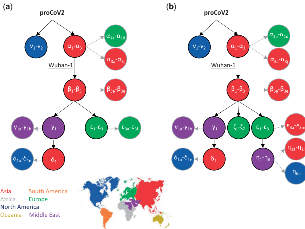
Fig. 4. The backbone of SARS-CoV-2 mutational history. The mutational history inferred was from (a) 29KG and (b) 68KG data sets. Major variants and their mutational pathways are shown in black, and minor variants and their mutational pathways are shown in gray. Circle color marks the region where variants were sampled first. The 68KG data set contains 12 additional variants and more than two times the genomes than the 29KG data set.
