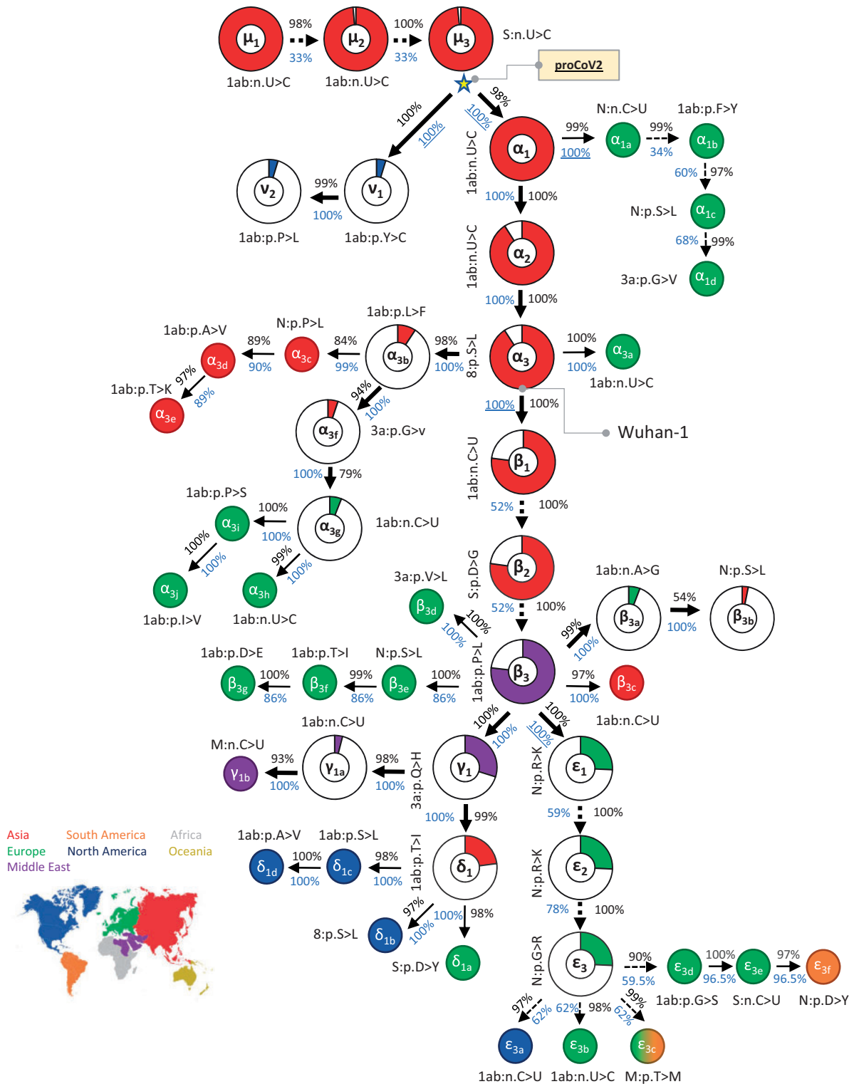
Fig. 2. Mutational history graph of SARS-CoV-2 from the 29KG data set. Thick arrows mark the pathway of widespread variants (frequency, v_f \geq 3\% ), and thin arrows show paths leading to other common mutations ( 3\% > v_f > 1\% ). The pie-chart sizes are proportional to variant frequencies in the 29KG data set, with pie-charts shown for variants with v_f > 3\% and pie color based on the world's region where that mutation was first observed. A circle is used for all other variants, with the filled color corresponding to the earliest sampling region. The COI (black font) and the BCL (blue font) of each mutation and its predecessor mutation are shown next to the arrow connecting them. Underlined BCL values mark variant pairs for which BCLs were estimated for groups of variants (see Materials and Methods) because of the episodic nature of variant accumulation within groups resulting in lower BCLs ( < 80\% , dashed arrows). Base changes (n.) are shown for synonymous mutations, and amino acid changes (p.) are shown for nonsynonymous mutations along with the gene/protein names ("ORF" is omitted from gene name abbreviations given in table 1). More details on each mutation are presented in table 1.
