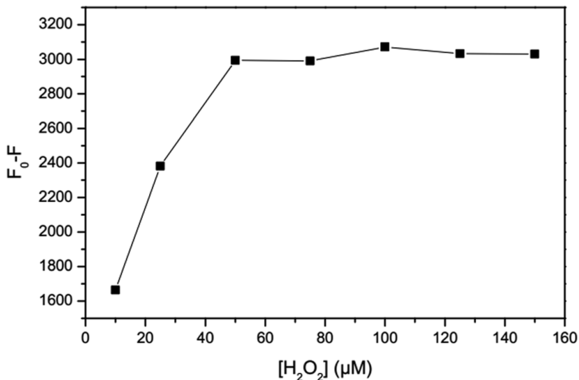
Fig. 5 Effect of \text{H}_2\text{O}_2 concentration.
