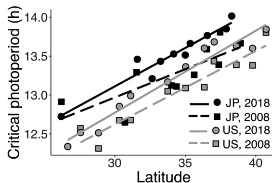
Figure 2 Relationship between diapause timing and latitude in Japan and US, 2008 and 2018. Critical photoperiod strongly correlates with latitude in populations from the United States and Japan in 2008 and 2018, forming parallel lines. Longer latitude-specific critical photoperiods in Japan compared to the United States imply entry into diapause earlier in the season, despite the later date of first frost (Fig. 1b); this difference between clines was present in both 2008 and 2018. Lines represent linear regressions; see Table 1
