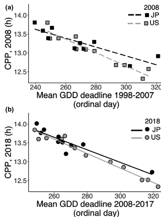
Figure 4 GDD deadline explains CPP across continents. Critical photoperiod measured in the lab for mosquitoes collected in 2008 (a) and 2018 (b) at multiple sites (each point on the graph). The measured CPP for each population is compared to the mean GDD-465 deadline calculated from climate data and expressed as an ordinal day of the year after which individuals must lay diapause eggs to avoid early termination of development and loss of fitness. GDD values are the average across years in the preceding decade for each time period. A similar correlation is found with GDD-465 deadline in the previous single year (Fig. S6; Table S3). Timing of diapause entry as represented by critical photoperiod thus correlates with the date in each location when insufficient growing degree days remain to complete another generation in the season, regardless of country of population origin. These results show that differences in latitude-specific GDD-465 between countries account for differences in latitude-specific CPP between countries. Lines represent results of linear regression; see Table 2 for test statistics
