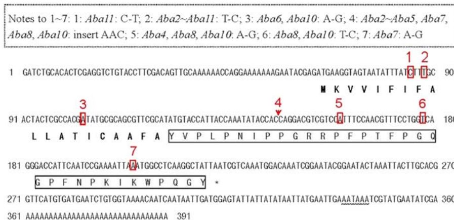
Figure 3. Nucleotide sequence and predicted amino acid sequence of Abaecin1 (GenBank Accession EU714043). The putative signal peptide is bolded, and the mature peptide is indicated by an open box. The translational signal (TAA) is indicated by the star symbol. Restriction and poly (A) adenylation signals (AATAAA) are indicated by a wavy line. The variant loci are boxed or indicated in red by a short arrow, and numbered in red. The nucleotide substitution sites in the precursor sequences between Abaecin1 and other Abaecin genes are boxed with a dotted line. “ Abaecin1~Abaecin11 ” is abbreviated to “ Aba1~Aba11 ”.
