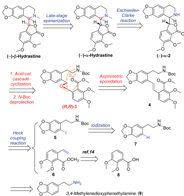
Scheme 3 Retrosynthetic analysis of (–)-β-hydrastine.
