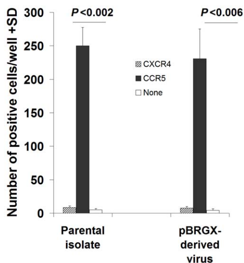
Figure 4. Co-receptor-mediated tropism of the pBRGX construct and its parental primary isolate. U373-MAGI-CXCR4 cem (CXCR4), U373-MAGI-CCR5e (CCR5) and U373MAGI (none) cells were infected with either pBRGX-derived virus or its parental primary isolate. The infectivity of the virus was tested by the X-Gal Staining assay. The number of positives were scored per well and indicated along the y-axis.
