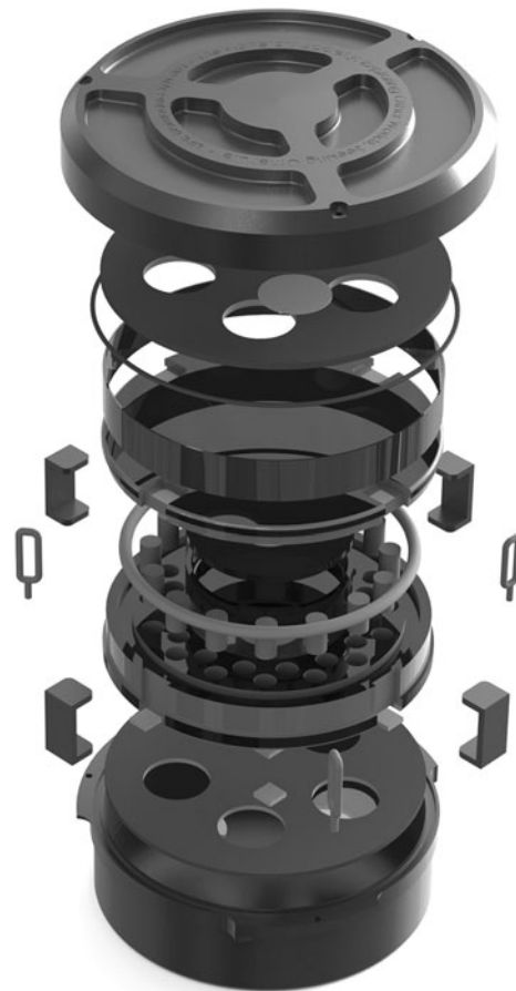
FIG. 2. Exploded view of Phobos LIFE biomodule showing components.
