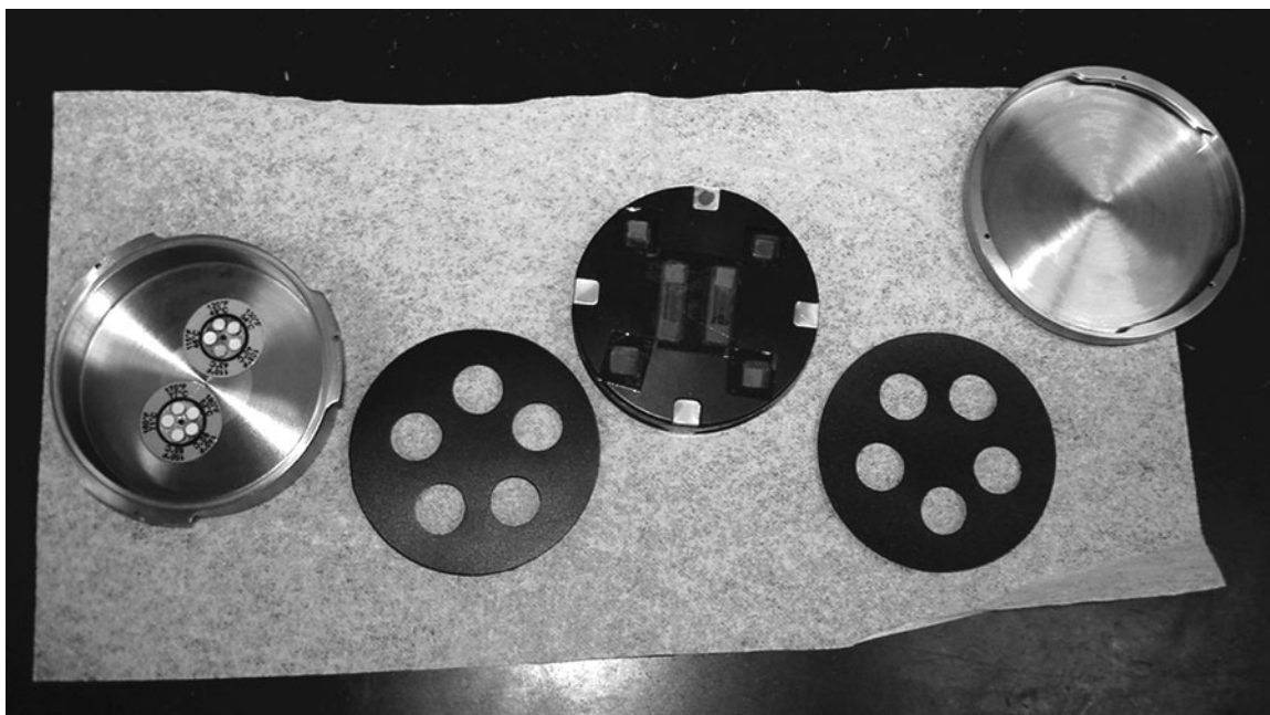
FIG. 5. Biomodule during assembly. Left to right: Titanium bottom with two temperature sensors, shock pad, bottom of loaded carrier including TLD radiation detectors (small white squares under Kapton tape), shock pad, and titanium lid.
