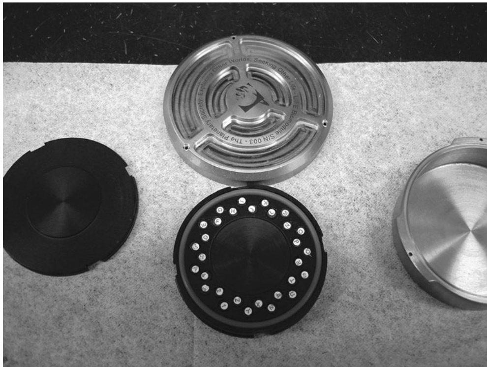
FIG. 4. Lower half of Delrin carrier (center) loaded with labeled sample tubes and central soil container. Note silicone O-ring. Also, top of carrier (left), titanium lid (top), and titanium bottom (right).
