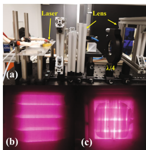
Fig. 3. Laser optics. (a) One of the two setups: The laser is a 4x60W stack with Volume Bragg Grating built-in to narrow the bandwidth, a quarter-waveplate to produce circular polarisation of the laser light, and lenses to shape the beam profile to cover the optical pumping cell. (b) Laser profile at the entrance of the oven. (c) Projected laser profile after the OPC. The vertical streaks are due to lensing by the uneven glass wall of the blown Ge-180 cell.
