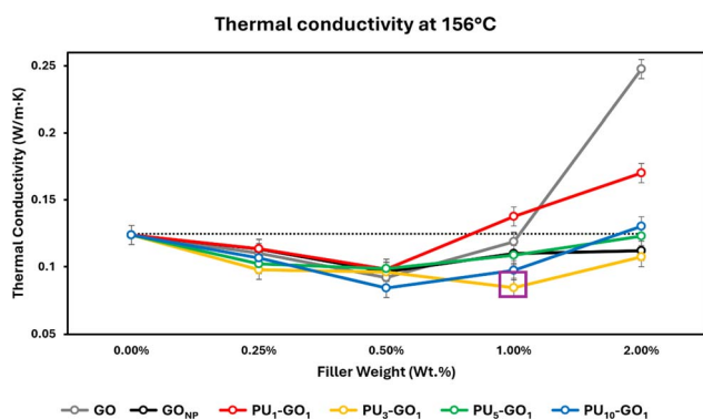
Fig. 3 Thermal conductivity of PU foams with varying weight percentages of each filler. It is important to note that lower thermal conductivity indicates a greater capacity for thermal insulation. A purple box is drawn around PU 3 -GO 1 1.0%, the only sample where the lowest thermal conductivity did not occur at 0.5% filler content.
