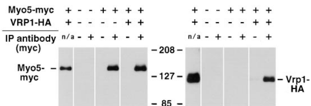
Figure 11. Vrp1p coimmunoprecipitates with Myo5p. Yeast strains that express no tagged constructs (HA10-1b), myc-tagged Myo5p (HA31-9c bearing pMYO5 ), or myc-tagged Myo5p and HA-tagged Vrp1p (VHA-1 bearing pMYO5 ) were grown to mid-log phase, disrupted, and then subjected to immunoprecipitation in the presence and absence of anti-myc antibody. Recovery of myc-tagged Myo5p was confirmed by Western blot analysis using anti-myc antibodies ( left ). Coimmunoprecipitation of HA-tagged Vrp1p with myc-tagged Myo5p was evaluated by decorating the same blot with anti-HA antibodies ( right ). The first lanes of each blot are whole cell lysates from VHA-1 bearing pMYO5 that illustrate the presence and electrophoretic mobility of tagged proteins.
