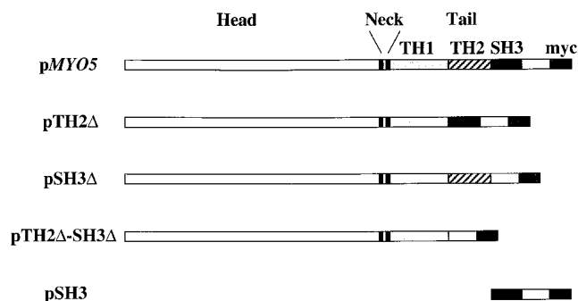
Figure 1. Schematic diagram of Myo5p mutants. pMYO5 , plasmid-borne wild-type MYO5 gene bearing three copies of the myc epitope at its carboxy terminus; pTH2Δ , plasmid-borne, myc-tagged MYO5 gene bearing a deletion of the TH2 region; pSH3Δ , plasmid-borne, myc-tagged MYO5 gene bearing a deletion of the SH3 region; pTH2Δ-SH3Δ , plasmid-borne, myc-tagged MYO5 gene bearing deletions of the TH2 and SH3 regions; pSH3 , plasmid-borne, myc-tagged SH3 domain of MYO5 gene. With the exception of pSH3 , all constructs were expressed in myo3Δ myo5Δ mutant cells. pSH3 was expressed in the myo3Δ strain. All proteins were expressed under control of the MYO5 promoter.
