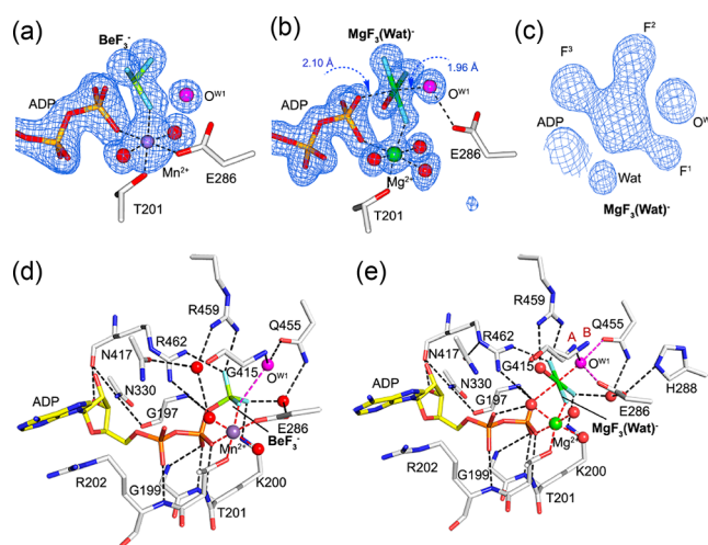
Figure 2. Omit maps ( mF_o - DF_c ) of (a) NS3h-MnADP-BeF 3 - and (b) NS3h-MgADP-MgF 3 (Wat) - complexes contoured at 4σ and (c) at 8σ. Active site interactions of (d) the NS3h-MnADP-BeF 3 - and (e) the NS3h-MgADP-MgF 3 (Wat) - complexes.
