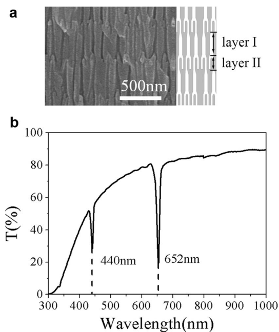
Figure 1 | SEM images and Transmittance of the as-prepared PC. (a) Periodic structure of the AAO based PC (left), and schematic illustration (right) in which the white part is air pore and the gray part is alumina. (b) Transmittance spectrum of the as-prepared AAO based PC.
