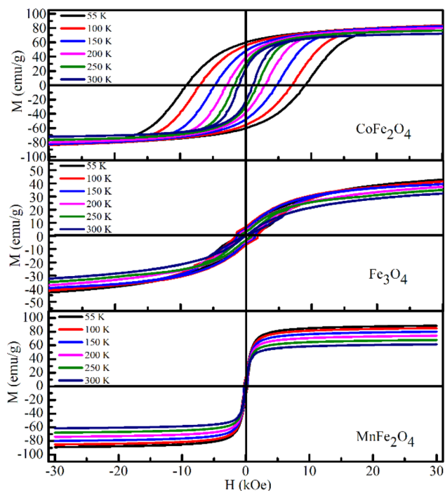
Fig. 11 M(H) loops measured at different temperatures for the M\text{Fe}_2\text{O}_4 system.
