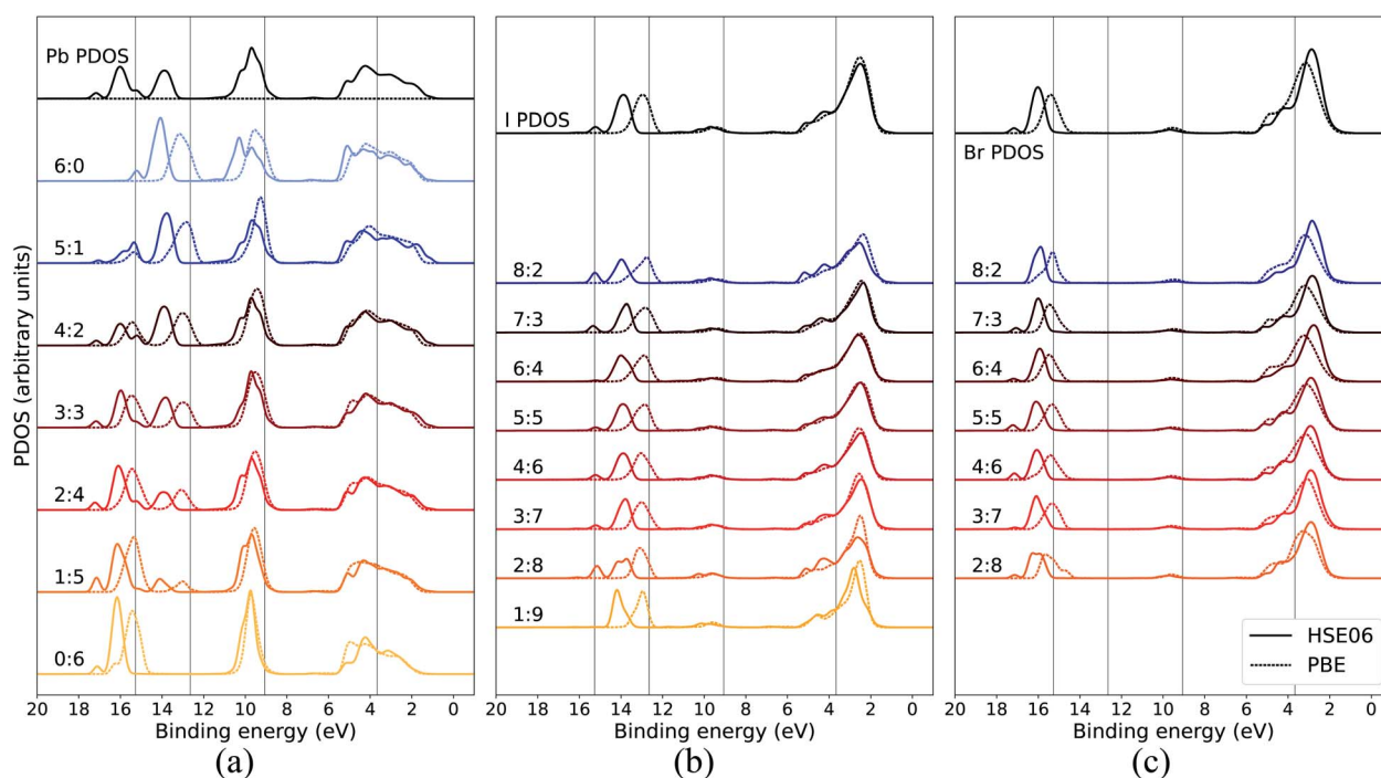
Fig. 5 Local coordination and local electronic structure using the PBE GGA functional and the HSE06 hybrid functional, shown in dashed and solid lines respectively, of \text{CH}_3\text{NH}_3\text{Pb}(\text{I}_{0.5}\text{Br}_{0.5})_3 for (a) Pb, (b) I, and (c) Br. The same energy shift (see Methods section) as in Fig. 2 was used for the GGA results while the HSE06 PDOS was shifted by 1.245 eV. The PBE results for local environments at x = 0.5 are reproduced from Fig. 3(b), 4(a) and (b).
