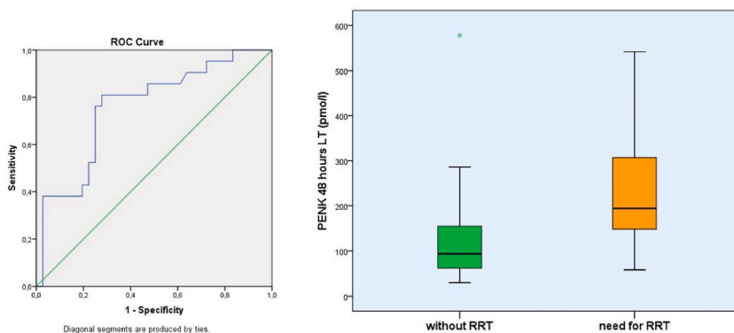
Fig. 4. ROC curve AUC and levels of PENK 48 h after LT in the need-RRT groups.
