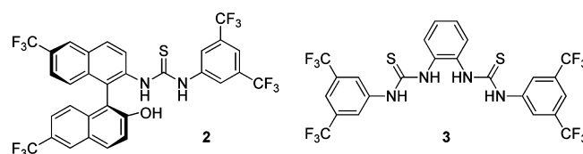
Figure 1. Structure of thioureas 2 and 3 employed as catalysts or templates in [2 + 2] photocycloaddition reactions.
