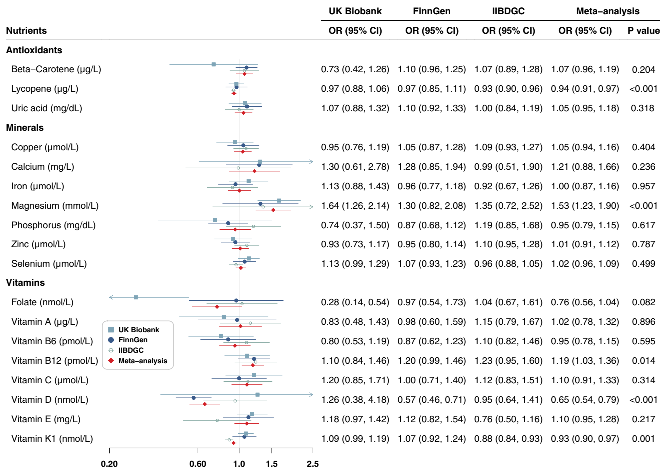
FIGURE 2 Associations of antioxidants, minerals and vitamins with risk of Crohn's disease. CI, confidence interval; OR, odds ratio.
