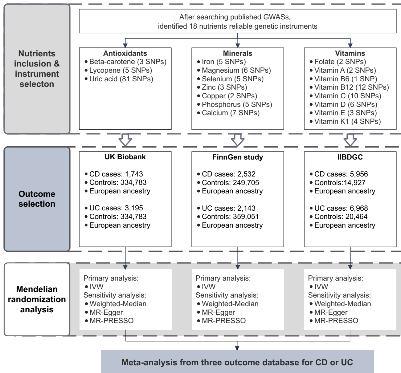
FIGURE 1 A flowchart of study design. CD, Crohn's disease; UC, ulcerative colitis; IIBDGC, The International Inflammatory Bowel Disease Genetics Consortium; IVW, inverse-variance weighted; MR-PRESSO, MR Pleiotropy RESidual Sum and Outlier.
