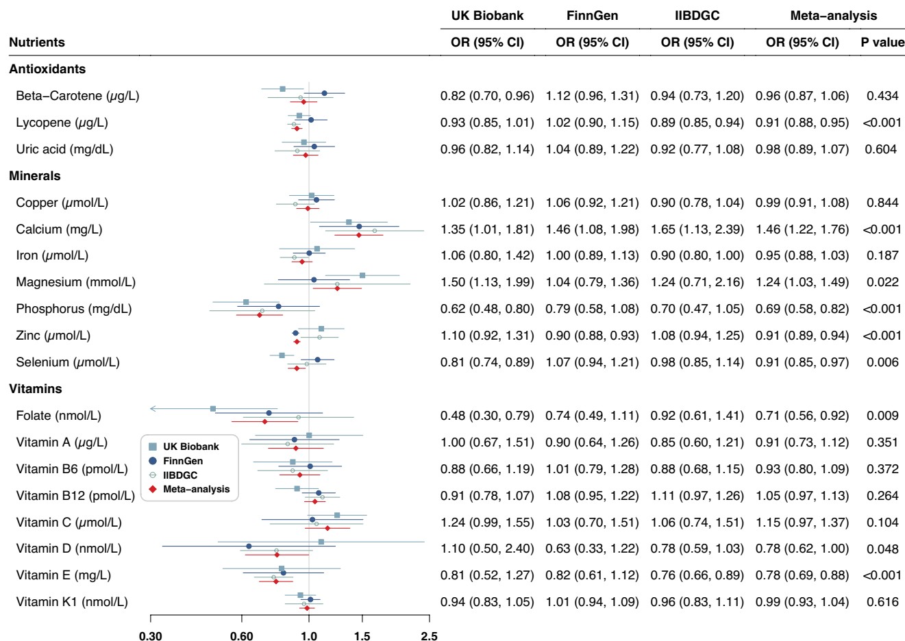
FIGURE 3 Associations of antioxidants, minerals and vitamins with risk of ulcerative colitis. CI, confidence interval; OR, odds ratio.
