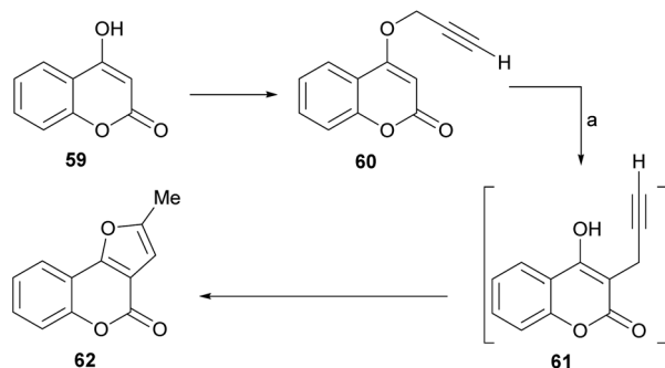
Scheme 5 Reagents and conditions: (a) HCONHMe, MW, 18 min (65%), or HCONHt, 14 h, reflux (52%).
