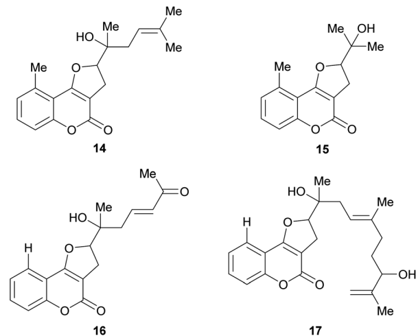
Fig. 4 Naturally occurring furo[3,2-c]coumarins carrying a tertiary alcohol motif.
