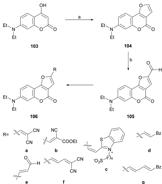
Scheme 23 Reagents and conditions: (a) (1) \text{ClCH}_2\text{CHO} , \text{K}_2\text{CO}_3 , \text{H}_2\text{O} , 0^\circ\text{C} ; (2) 40% HCl, (b) DMF, \text{POCl}_3 , 70^\circ\text{C} (45% overall).
