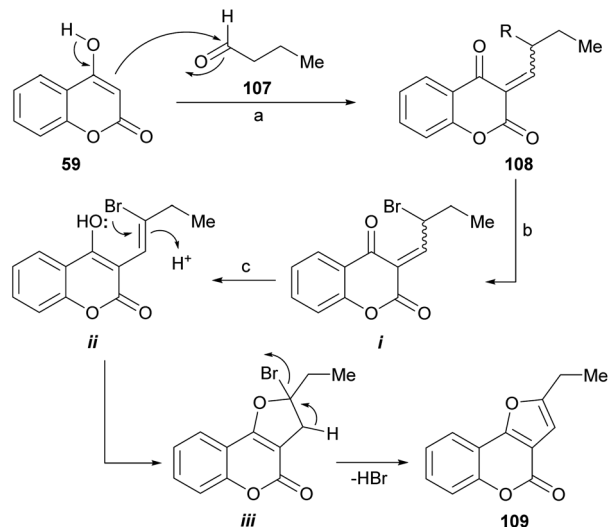
Scheme 24 Reagents and conditions: (a) \text{TsOH} (5 mol%), MeCN; (b) NBS, MeCN; (c) \text{TsOH} , MeCN, 80^\circ\text{C} , 2 h (33%).
