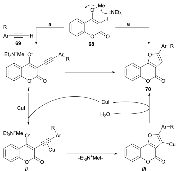
Scheme 9 Reagents and conditions: (a) 69 , Pd(PPh 3 ) 2 Cl 2 (cat.), Cul (cat.), Et 3 N, MeCN, 60 °C, 15 h (70%).
