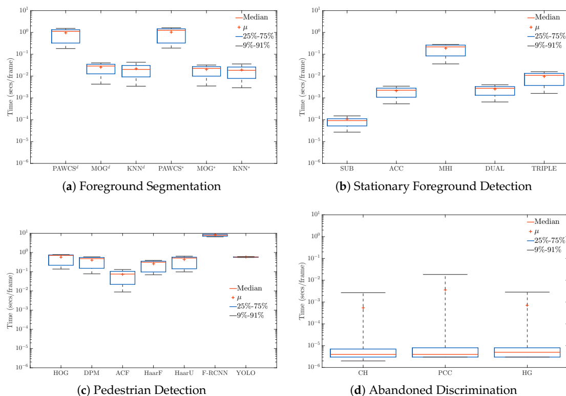
Figure 15. Computational cost analysis, in terms of seconds per frame, of every algorithm implemented at each stage: Foreground Segmentation (a), Stationary Foreground Detection (b), Pedestrian Detection (c) and Abandoned Discrimination (d).
