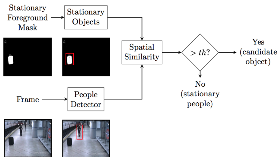
Figure 6. Block diagram of the candidate generation module. Stationary objects and people detection blobs are independently extracted and then spatially compared. If a stationary object overlaps with people detection, it is considered as a static person, otherwise the object is a potential abandoned object candidate.
