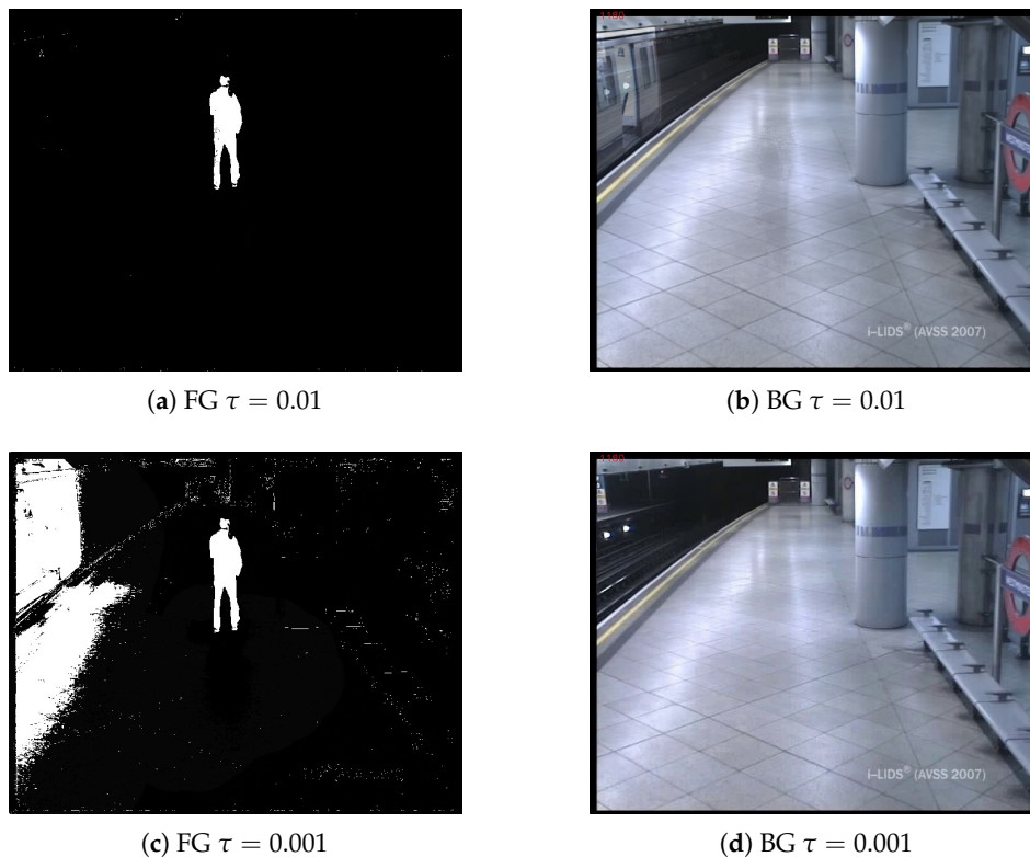
Figure 3. Examples of different adaptation rates for background subtraction based on the Mixture of Gaussians approach [45] for Frame 1180 of the sequence AVSS_AB_2007 ( http://www.eecs.qmul.ac.uk/~andrea/avss2007_d.html ). Subfigures (a,c) show Foreground (FG) masks with different parameter \tau , which controls the update rate of the Background (BG) models, that are depicted in subfigures (b,d).
