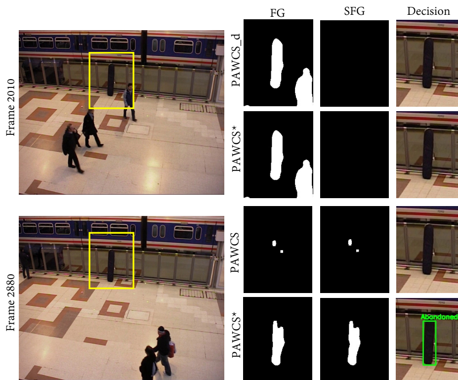
Figure 10. Columns from left to right show the frame image with event ROI marked in yellow, foreground mask, static foreground mask, and final decision. The first and second row show visual results at different stages of Frame 2010, when the object has just been left. Both default and tuned PAWCS detect the object as part of the foreground; however, for a further frame (third and fourth rows), only tuned PAWCS maintains the object detection, while default PAWCS misses the abandoned object.
