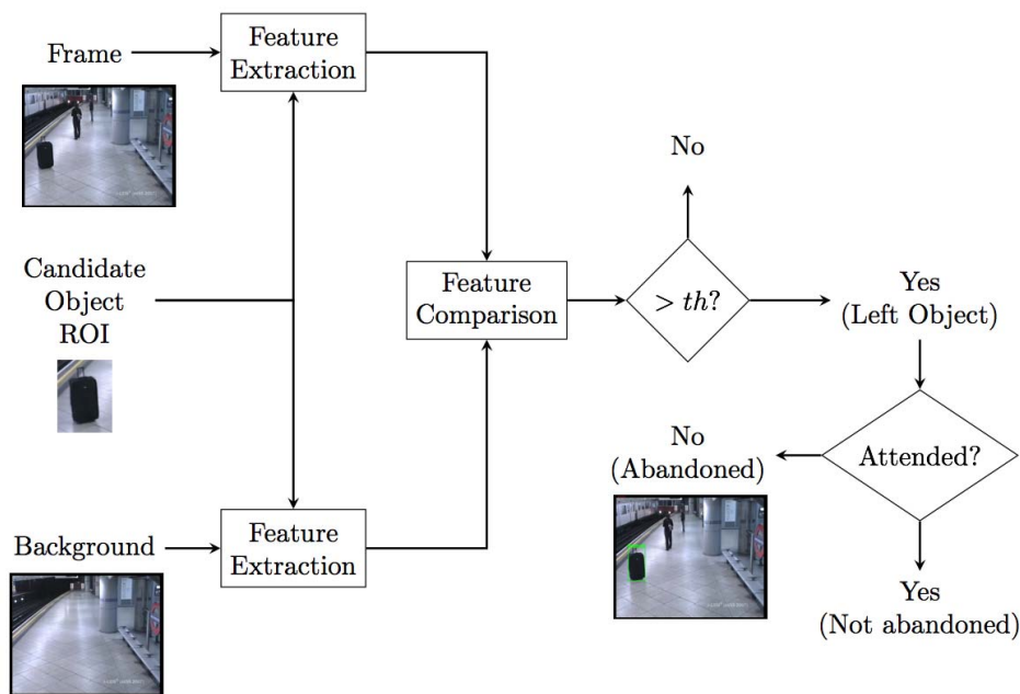
Figure 7. Block diagram of candidate validation module. In simple terms, for each candidate, its region of interest is extracted, and certain features are extracted comparing them with the background and current frame. Through this comparison, false objects are discarded. Finally it is checked if the object is attended.
