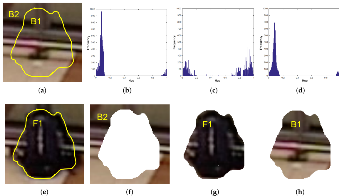
Figure 8. Example of Pixel Color Contrast algorithm operation. Subfigure (a) shows initial frame and (e) depicts an abandoned bag in a posterior frame. PCC computes Hue histograms, (b–d), from B2 (f), F1 (g) and B1 (h), respectively. Histogram comparisons (b,c) and (c,d) are made and final abandoned decision is taken from the results. Since (b) is more similar to (d) than to (c), this means (e) represents an abandoned object.
