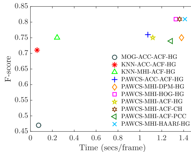
Figure 16. Relation between performance (F-score) and computational time (seconds per frame) of a selection of relevant configurations.
