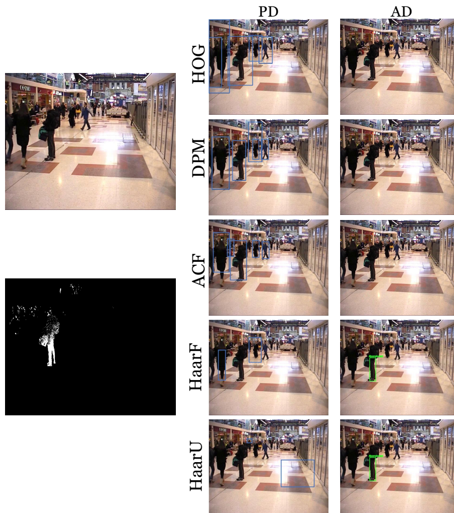
Figure 13. The first column shows the frame under consideration and its computed stationary foreground mask (DBM); the second column reports the visual results of the implemented people detector; and the third column presents the abandoned object discrimination of the system. It can be observed that the Haar-like feature classifier for full (HaarF) and upper body parts (HaarU) were not able to detect the standing stationary person; therefore, the system was mistakenly detecting him as an abandoned object.
