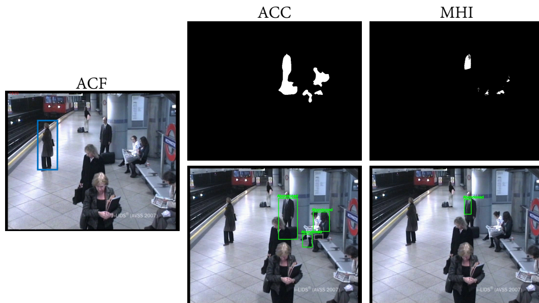
Figure 12. All images correspond to the same frame of the AVSS medium sequence. The image on the left shows in blue the detections provided by the ACF people detector. The top row illustrates the static foreground mask obtained with the ACC and MHI algorithms, respectively, and the bottom row shows their corresponding abandoned discrimination.
