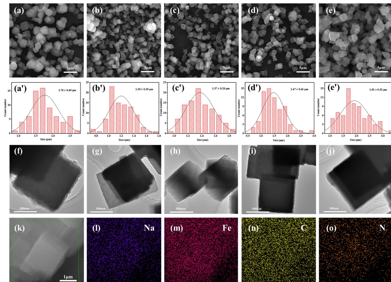
Fig. 3 SEM images of C-PB-0.3 (a), Y-PB-0.3 (b), Y-PB-15 (c), Y-PB-30 (d), and Y-PB-41 (e); particle size distribution graph of C-PB-0.3 (a'), Y-PB-0.3 (b'), Y-PB-15 (c'), Y-PB-30 (d'), and Y-PB-41 (e'); TEM images of C-PB-0.3 (f), Y-PB-0.3 (g), Y-PB-15 (h), Y-PB-30 (i), and Y-PB-41 (j); EDS mapping results of Y-PB-15 (k–o).
