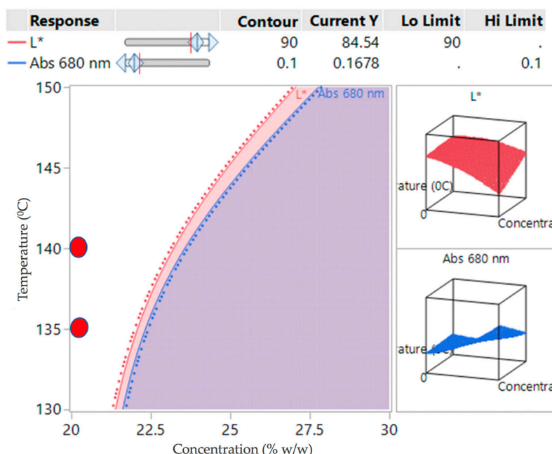
Figure 8. Contour plot for DoE2 indicating a potential design space (white region) overlaid verification study conditions (red circles).
