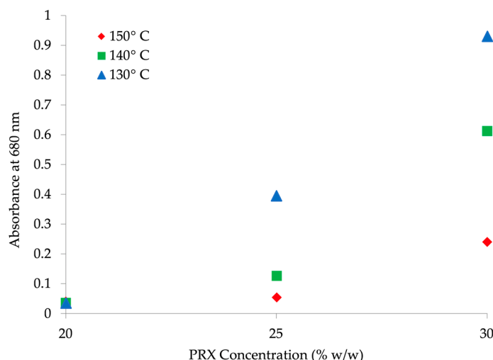
Figure 7. Absorbance at 680 nm vs. API concentration (% w/w) at 130 °C, 140 °C and 150 °C.
