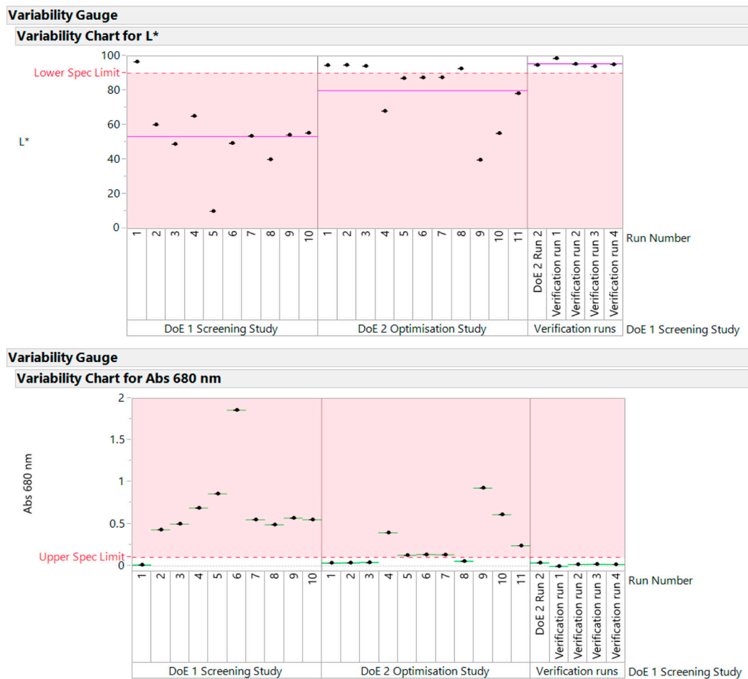
Figure 9. Variability gauge plot for data across all studies.
