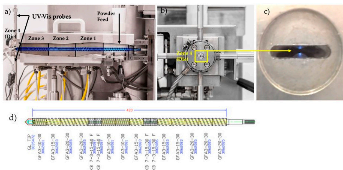
Figure 2. (a) Side view of the extruder; (b) Front view (zone 4 is where the UV-Vis probes are located), (c) View of the probes gap (0.5–0.8 mm) inside the zone 4; (d) standard screw configuration set (Leistritz Nano16 with co-rotating twin screws).
