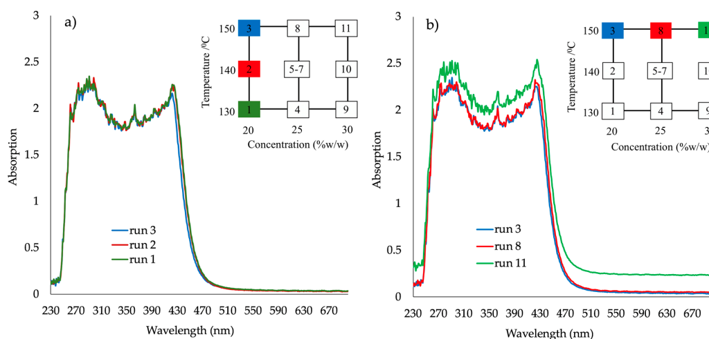
Figure 6. Absorbance spectra for the response surface design runs (DoE2) (a) API 20% w/w at 130 °C (run 1) 140 °C (run 2) and 150 °C (run 3); (b) temperature at 150 °C for API concentrations 20% w/w (run 3), 25% w/w (run 8) and 30% w/w (run 11).
