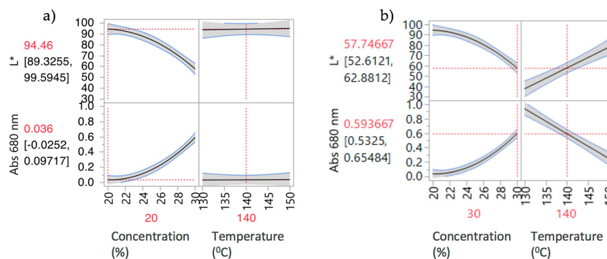
Figure 5. Prediction Profilers for DoE2 (a) 20% w/w and (b) 30% w/w concentrations.
