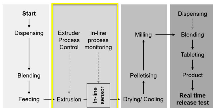
Figure 1. Schematic diagram showing the manufacturing process including the main unit operations from powders to final product, tablets [10]. The focus of this study is on the in-line UV-Vis monitoring of the hot melt extrusion (HME) process. Reproduced with permission from Lundsberg et al., Pharmaceutical Quality by Design: A Practical Approach ; published by Wiley, 2018.
