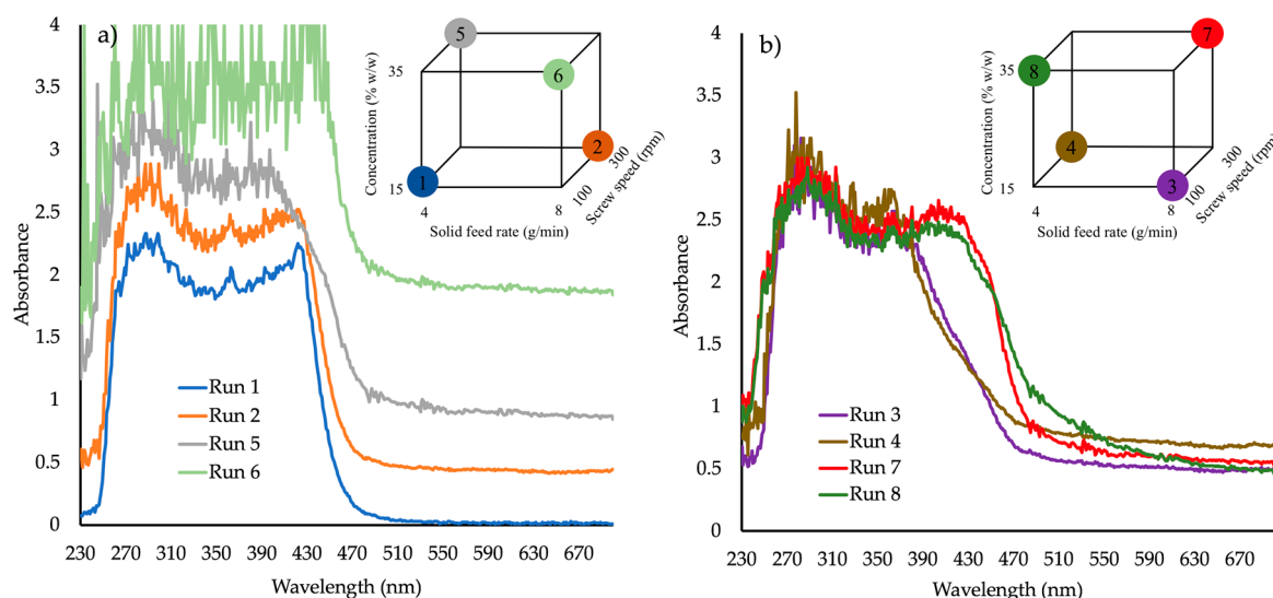
Figure 3. Absorbance vs. wavelength spectra for samples produced at (a) 150 °C and (b) 170 °C (DoE1, runs 1–8).
