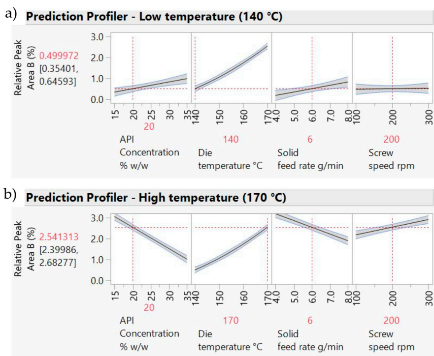
Figure 14. DoE model showing the impact of process parameters on the Relative area of Peak B. (a) Prediction profiler for 140 °C; (b) Prediction profiler for 170 °C
