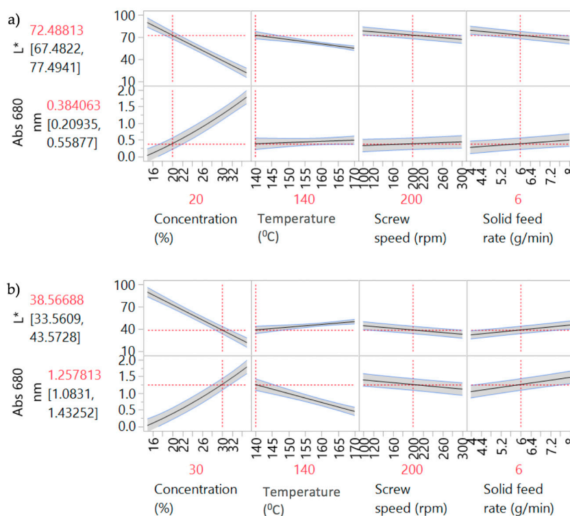
Figure 4. Prediction profilers for DoE1 for (a) 20% w/w and (b) 30% w/w PRX concentrations.
