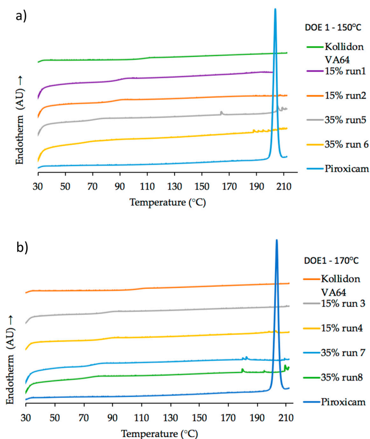
Figure 11. DSC heating curves ( 20\text{ }^\circ\text{C}/\text{min} ) of pure PRX, pure Kollidon ® VA64 as reference and samples from (a) DoE1 at 150\text{ }^\circ\text{C} ; (b) DoE1 at 170\text{ }^\circ\text{C} .
