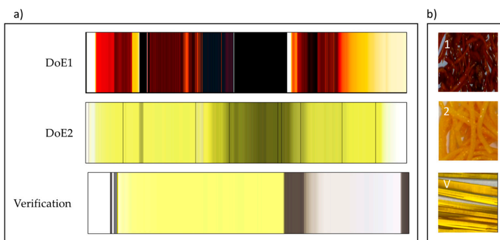
Figure 10. (a) Visualization of absorbance spectra of all experiments: DoE1, DoE2, verification. DoE1: \approx 2000 spectra collected in 5 h; DoE2: \approx 1500 spectra collected in 3 h; Verification: \approx 650 spectra collected in 2 h. (b) Representation of samples from each DoE showing color and appearance of extrudates: (1) DoE1 opaque and very dark red (run 6: API 35% w/w , T = 150 °C, 100 rpm, 8 g/min); (2) DoE2 opaque and slightly orange (run 10: API 30% w/w , T = 140 °C, 200 rpm, 6 g/min); (V) Verification, transparent light yellow (run: API 20% w/w , T = 140 °C, 200 rpm, 6 g/min). Reproduced with permission from Lundsberg et al., Pharmaceutical Quality by Design: A Practical Approach ; published by Wiley, 2018.
