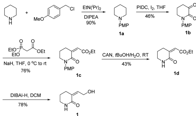
Scheme 1 Synthetic route of 1 .
