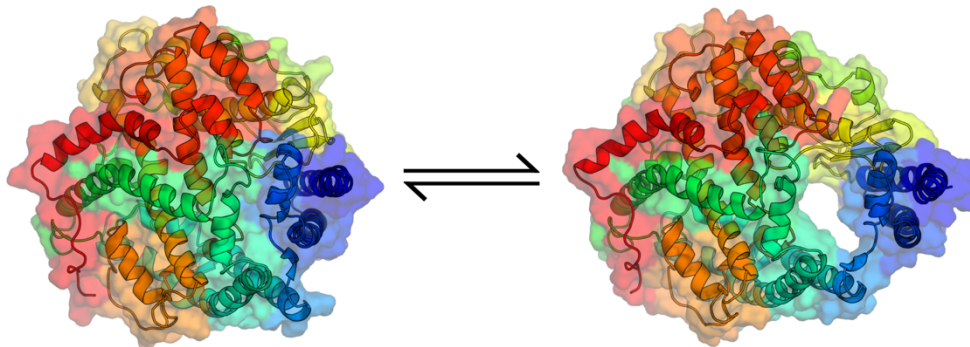
Figure S17: Human ACE2 transition from closed to open state. Backbone is represented as a cartoon and sidechains are represented with a transparent surface. The protein is colored by residue number following a rainbow. Pocket is proximal to the region that binds to SARS-CoV-2 spike protein.
