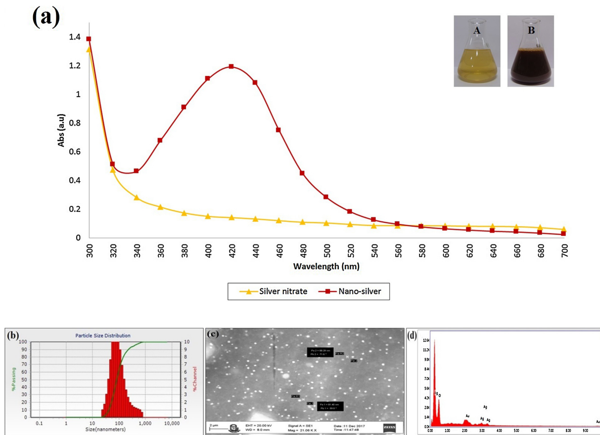
Fig. 1. Characterization of green synthesized nano-silver (a). UV–vis spectra (Inset: Colour changed before-A and after-B synthesis of nano-silver), (b). Particle size distribution by dynamic light scattering, (c). SEM image and (d). EDX spectrum (For interpretation of the references to colour in this figure legend, the reader is referred to the web version of this article).
